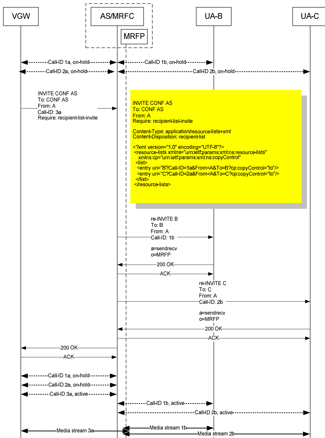
Figure C.6: Loose coupling 3PTY with INVITE method
