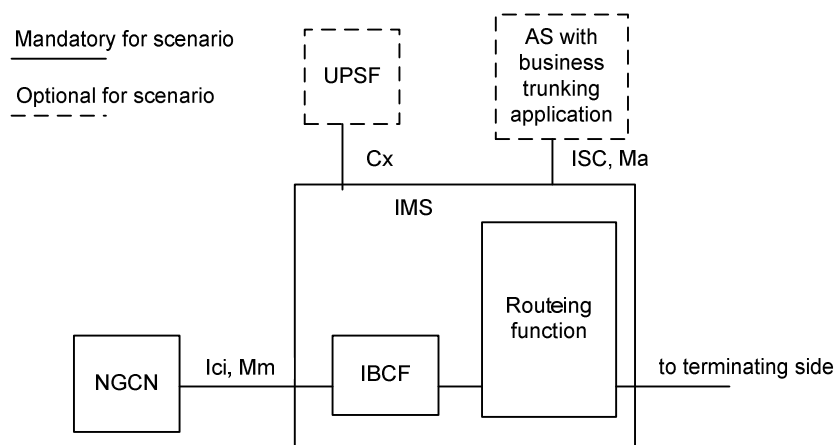
Figure 5.1: Originating Side with AS and UPSF
