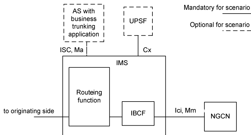
Figure 5.2: Terminating Side with AS and UPSF
