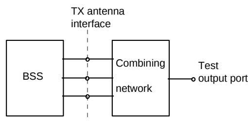
Figure 4.10-2: Transmitter test setup
