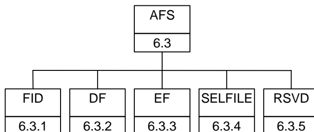
Figure 4: Breakdown of "AFS" Test Group
