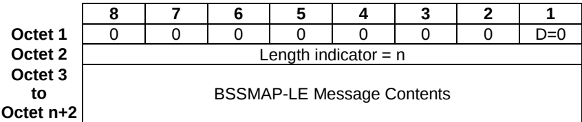
Figure 8.3.6-1: SCCP Data Field for a BSSMAP-LE Message
