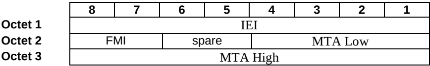
Figure 10.38.1: Multilateration Timing Advance Information
