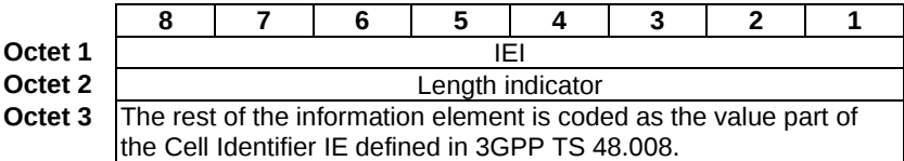
Figure 10.5.1: Cell Identifier IE
