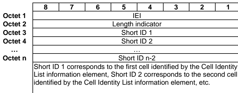
Figure 10.40.1: Short ID Set IE
