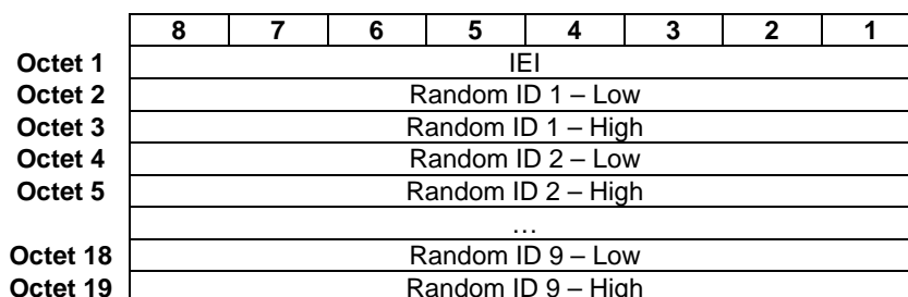
Figure 10.41.1: Random ID Set IE
