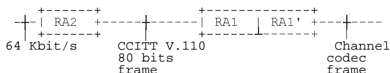
Figure 3GPP TS 48.060/4.2: Rate adaption when performed at the BTS.
