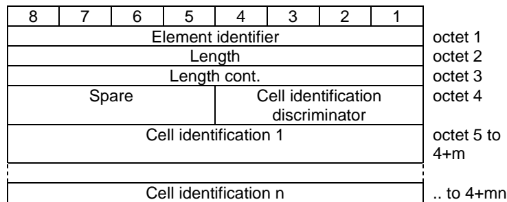
Figure 8.2.6.1: Cell List information element
