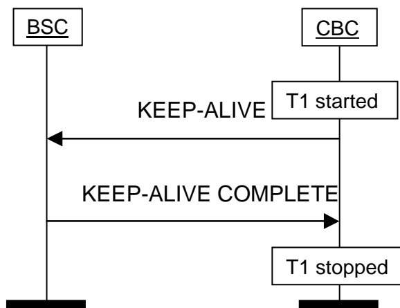
Figure 7.7a.2.1: Keep Alive Procedure: Successful Operation
