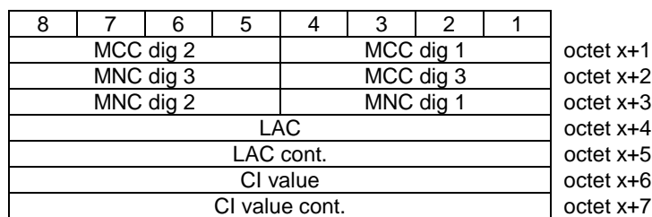
Figure 8.2.6.2: Coding of the i-th Cell Identification for Cell identification discriminator = 0000
