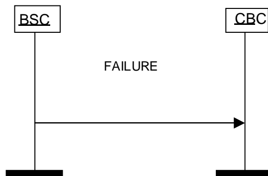
Figure 7.9.2.1: Failure Indication Procedure: Successful Operation
