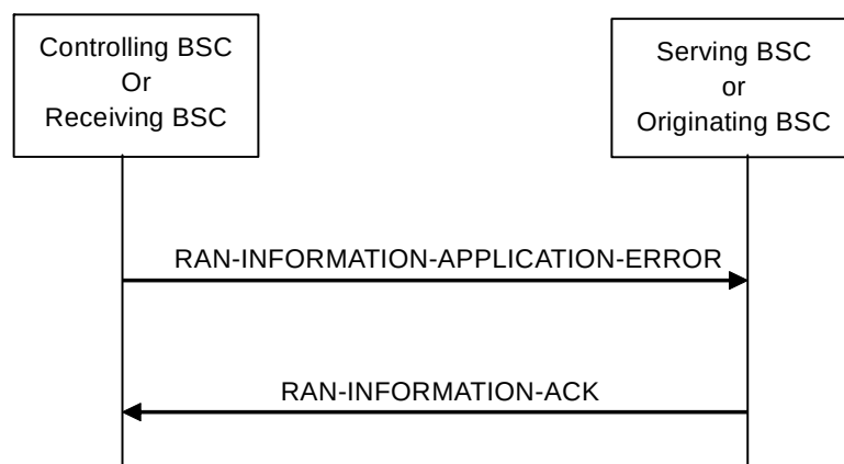
Fig 8c.2.4: RAN Information Application Error procedure
