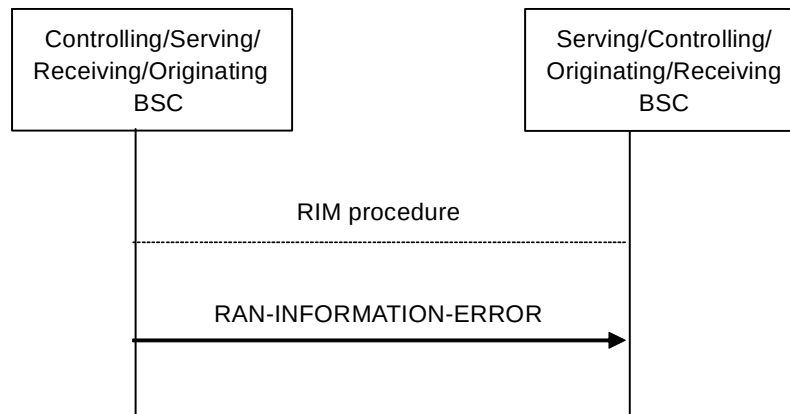
Fig 8c.2.5: RAN Information Error procedure
