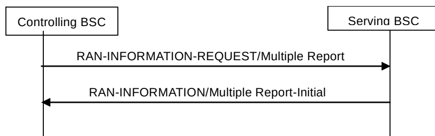
Figure 8c.2.2.2: Successful RAN Information Request/Multiple Report Procedure
