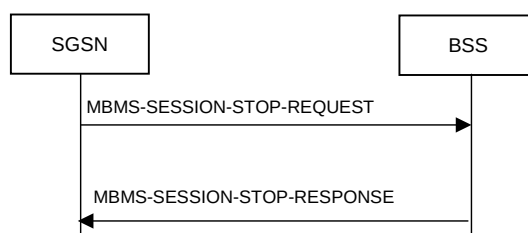
Figure 8d.3: MBMS Session Stop procedure
