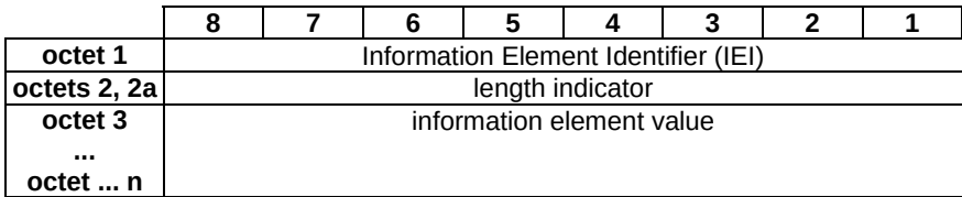
Figure 10.1.1: Information element structure, TLV format
