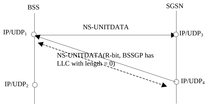
Figure B.3: Example 3 of NS entity requesting change flow without data
