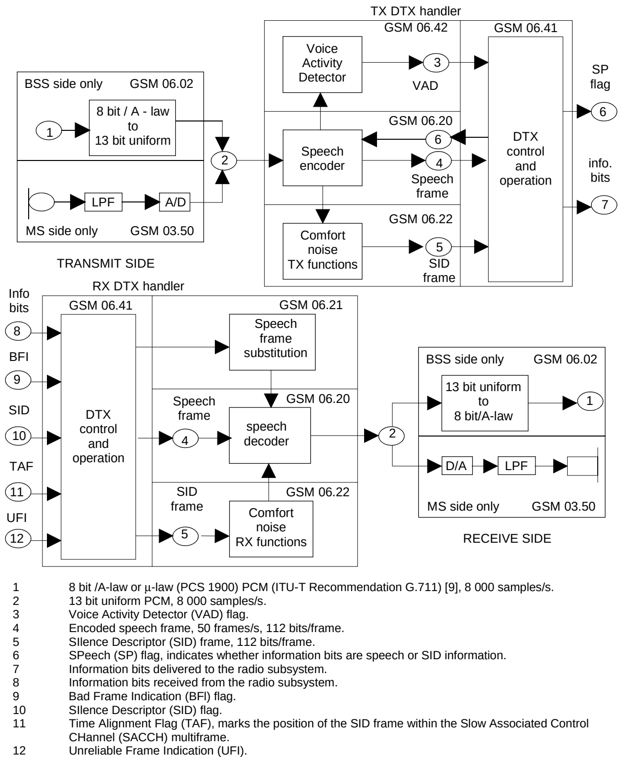
Figure 1: Overview of audio processing functions
