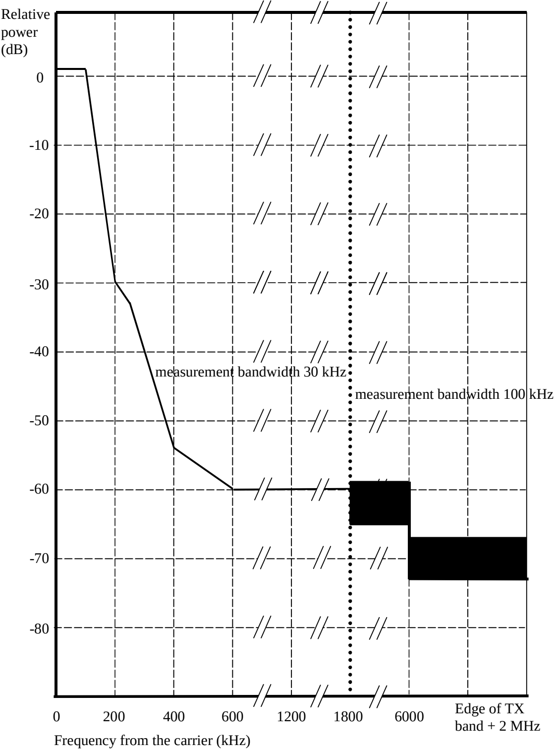
Figure A.3b: DCS 1 800 and PCS 1900 MS spectrum due to 8-PSK modulation, and 16-QAM with normal symbol rate
