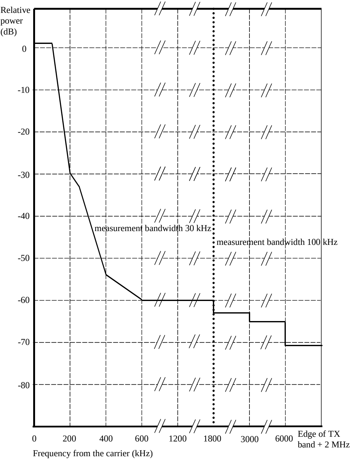
Figure A.1b: GSM 400, GSM 900, GSM 850 and GSM 700 MS spectrum due to 8-PSK modulation, and 16-QAM with normal symbol rate
