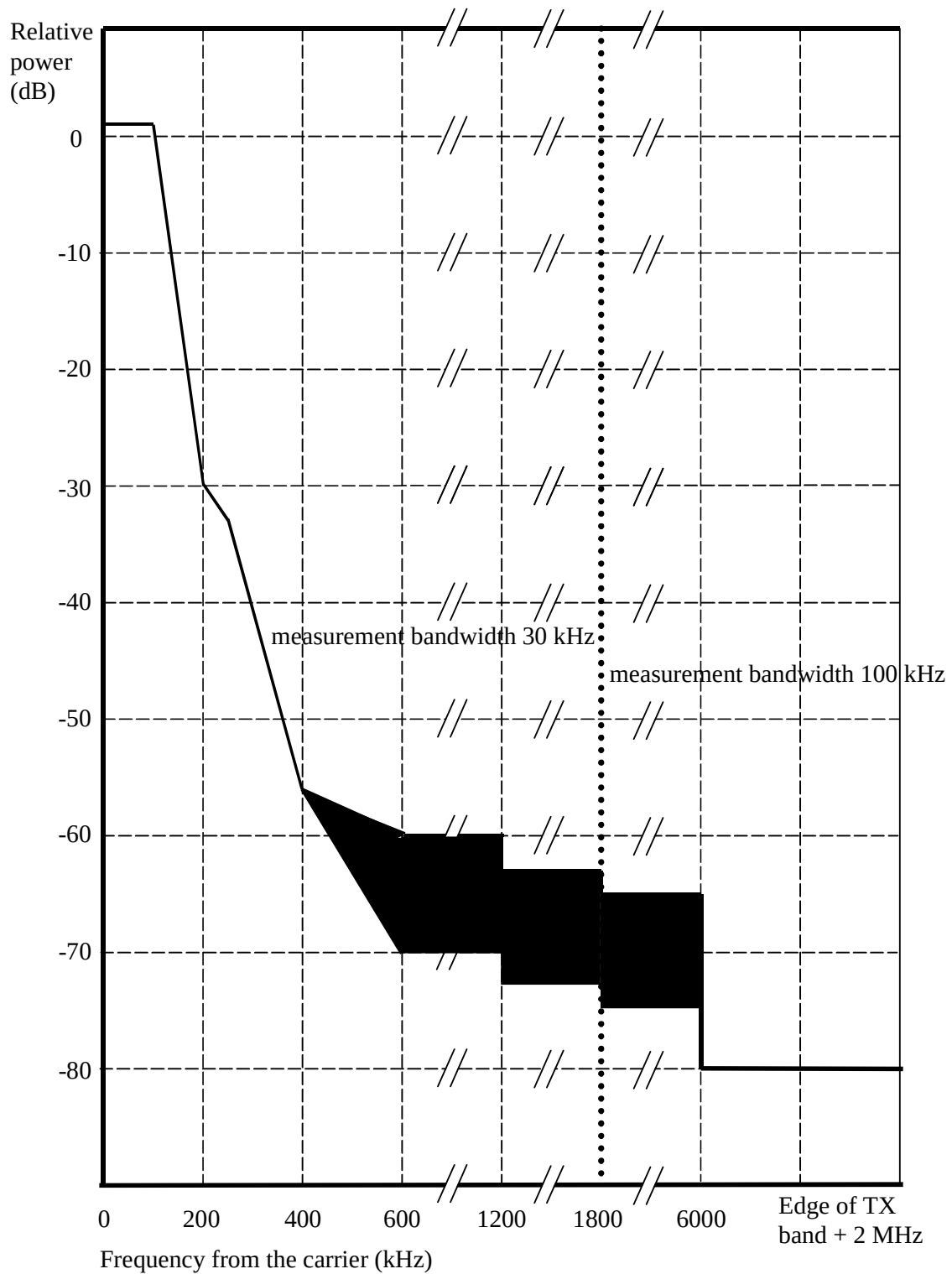
Figure A.2b: GSM 400, GSM 900, GSM 850, MXM 850, GSM 700, DCS 1800, PCS 1900 and MXM 1900 BTS spectrum due to 8-PSK modulation, and 16-QAM and 32-QAM with normal symbol rate
