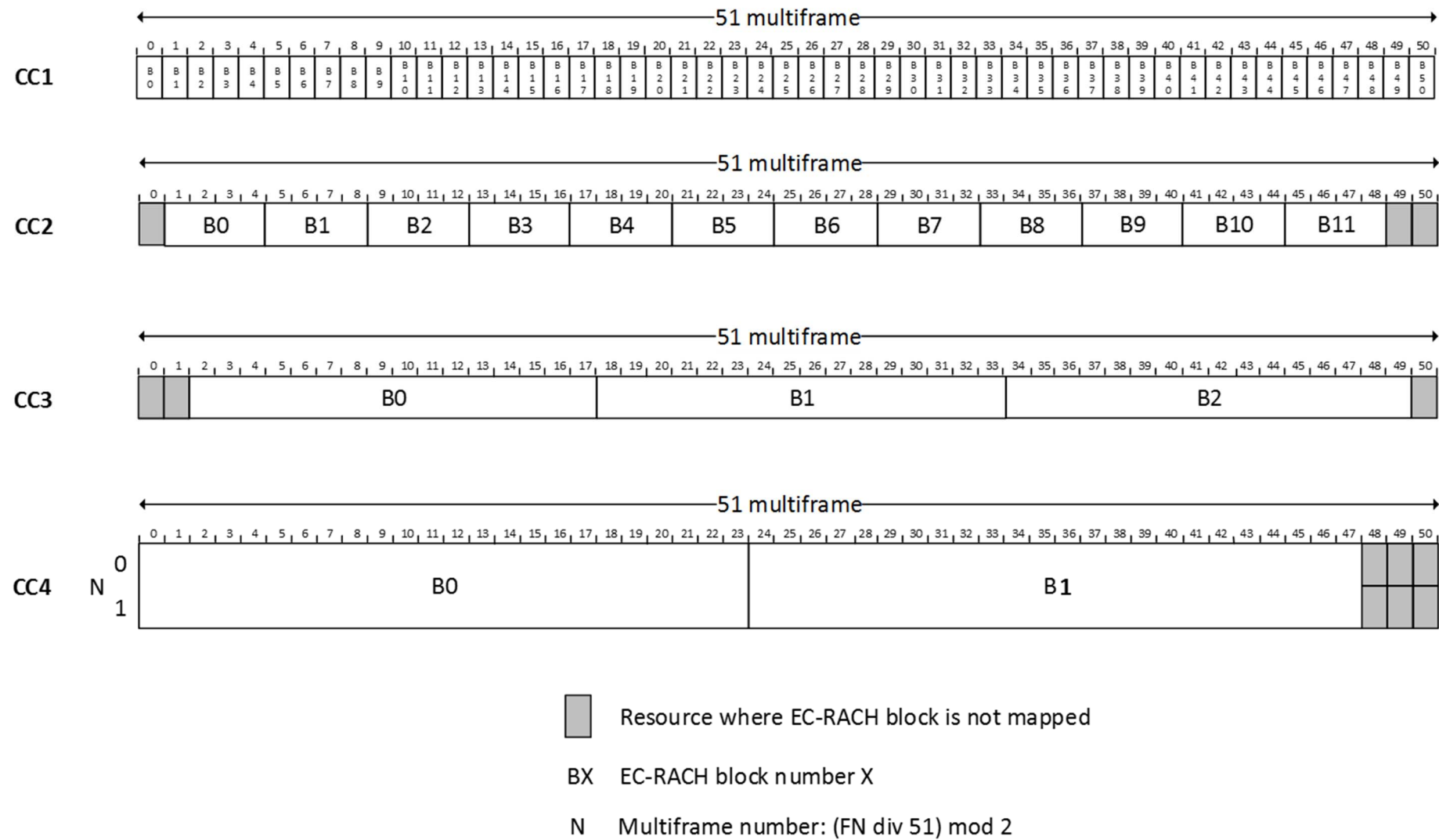
Figure 16: TDMA frame mapping for 1TS EC-RACH
