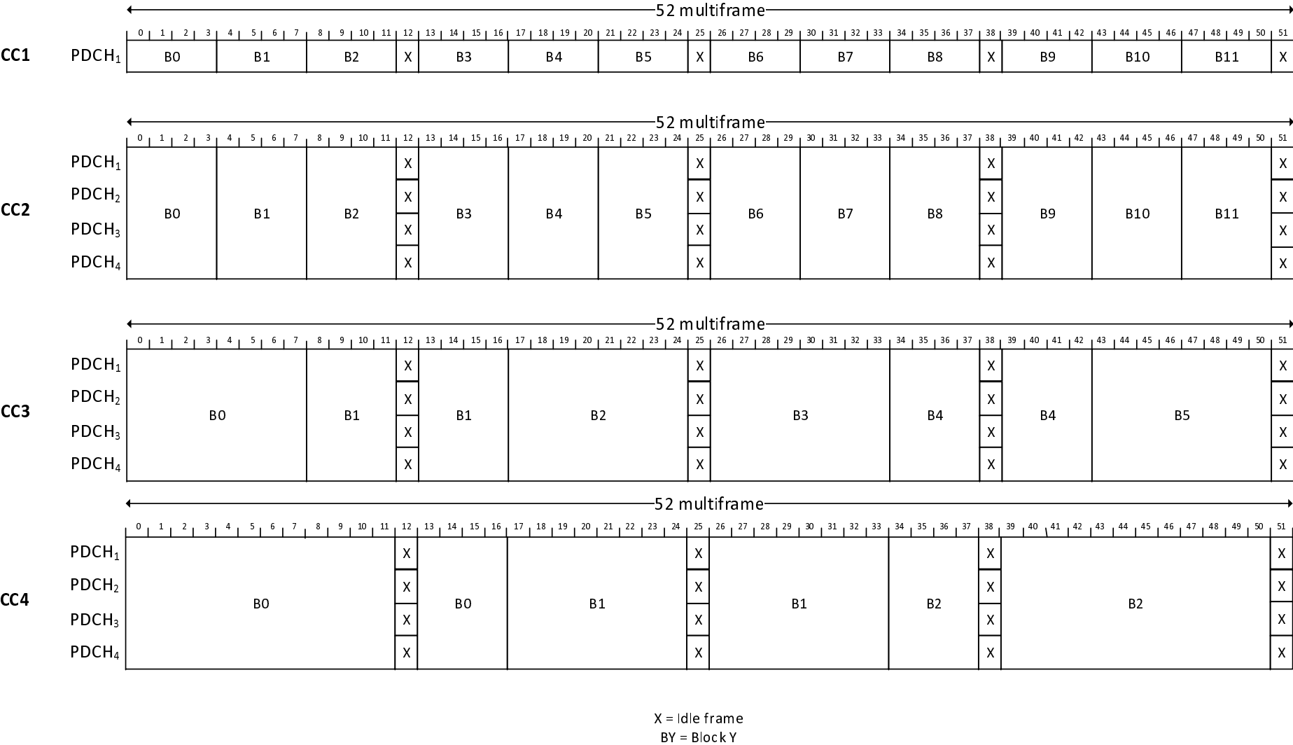
Figure 9b: 52-multiframe for EC-GSM-IoT for different Coverage Classes (CC) using 4 PDCHs for CC2 to CC4 in EC operation
