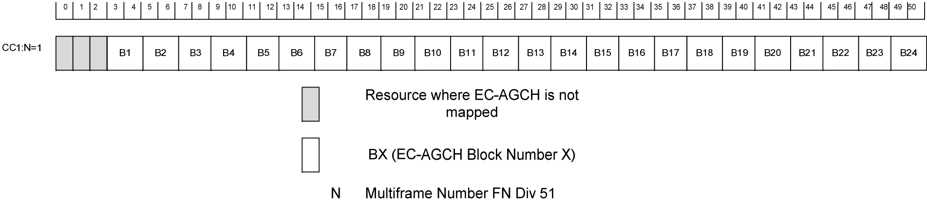
Figure 23: TDMA frame mapping for EC-AGCH for CC1 in TN3,TN5 and TN7 with EC-PICH configured
