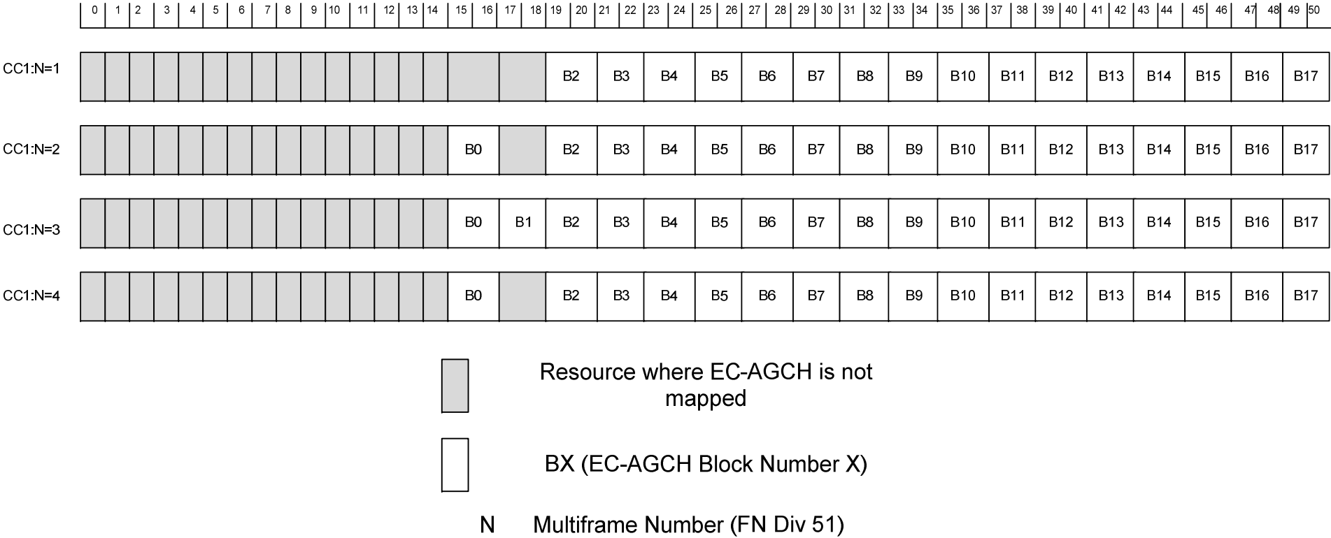
Figure 22: TDMA frame mapping for EC-AGCH for CC1 in TN1 with EC-PICH configured
