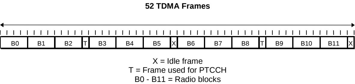
Figure 9: 52- multiframe for PDCHs in BTTI configuration
