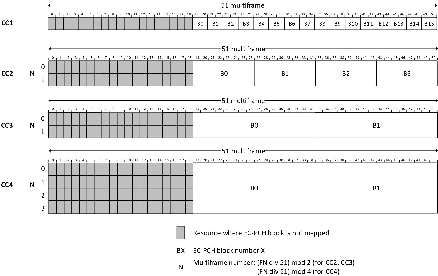
Figure 13: TDMA frame mapping for EC-PCH
