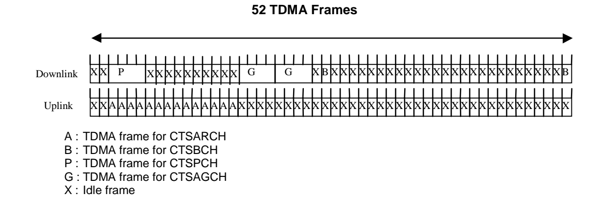
Figure 10: 52-multiframe for CTS
