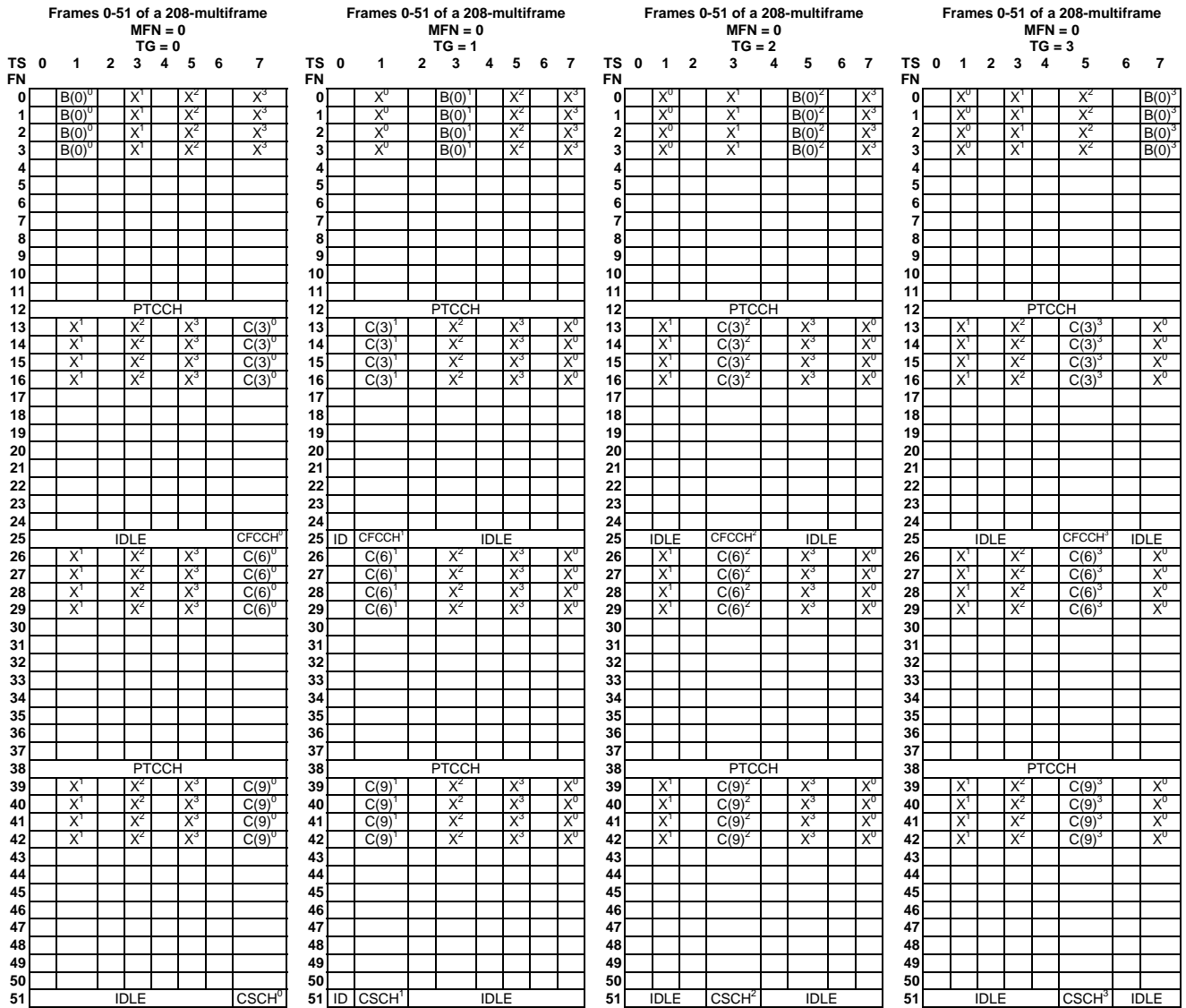
Figure D.1: COMPACT downlink 52-multiframe structure using 4 time groups for nominal cells (based on an assignment of 1 CPBCC and 3 CPCCCHs with NIB_CCCH_0 = NIB_CCCH_1 = NIB_CCCH_2 = NIB_CCCH_3 = 4). NIB_CCCH is not broadcast for serving cell time group
