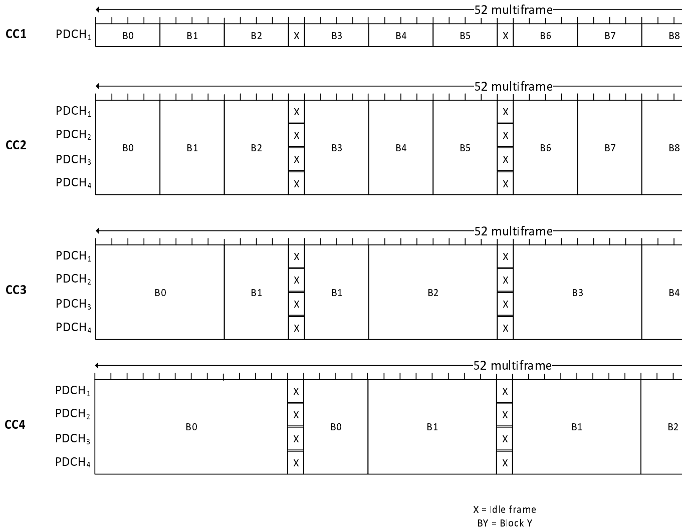
Figure 9b: 52-multiframe for EC-EGPRS for different Coverage Classes (CC)
