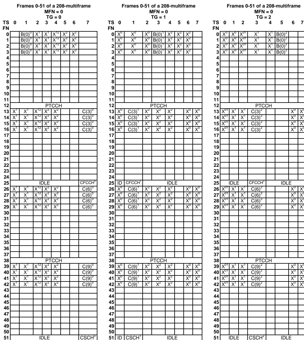
Figure D.4: COMPACT downlink 52-multiframe structure using 3 time groups for large cells (based on an assignment of 1 CPBCCCH and 3 CPCCCHs with NIB_CCCH_0 = NIB_CCCH_1 = NIB_CCCH_2 = 4, NIB_CCCH_3 = 0). NIB_CCCH is not broadcast for serving cell time group
