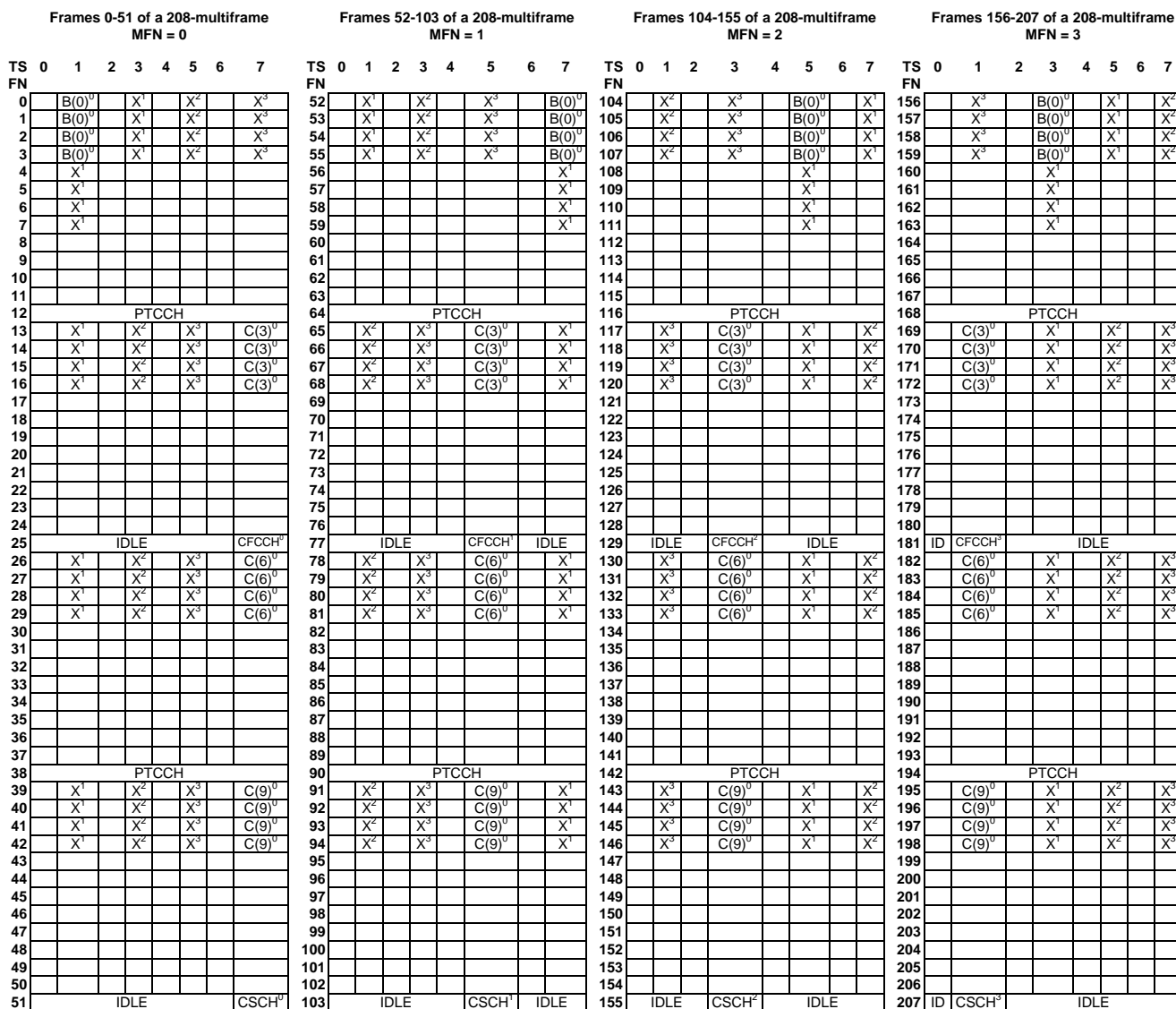
Figure D.7: Example of COMPACT downlink timeslot mapping and rotation of control channels using 4 time groups for nominal cells (based on an assignment of 1 CPBCCCH and 3 CPCCCHs with NIB_CCCH_0 = NIB_CCCH_2 = NIB_CCCH_3 = 4, NIB_CCCH_1 = 5). TG = 0 is illustrated. NIB_CCCH is not broadcast for serving cell time group
