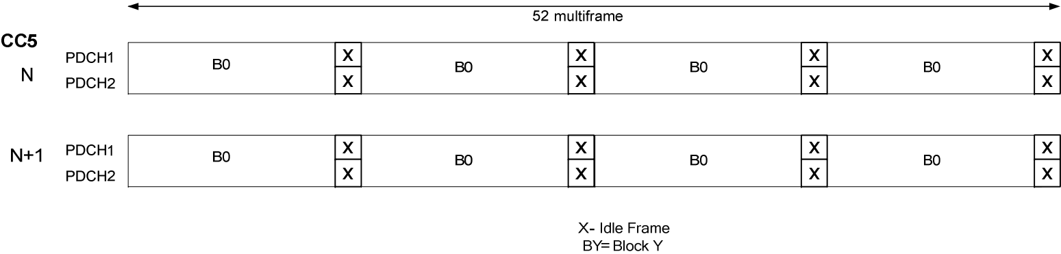
Figure 2a7: Multiframe structure for EC-GSM-IoT using two PDCHs for CC5 in EC operation.
