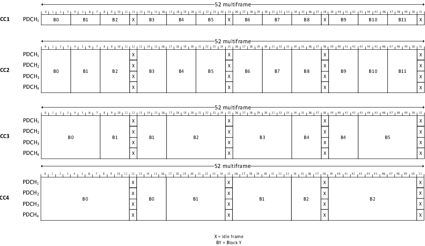
Figure 2a4: Multiframe structure for EC-GSM-IoT using one PDCH for CC1 and four PDCHs for CC2 to CC4 in EC operation.
