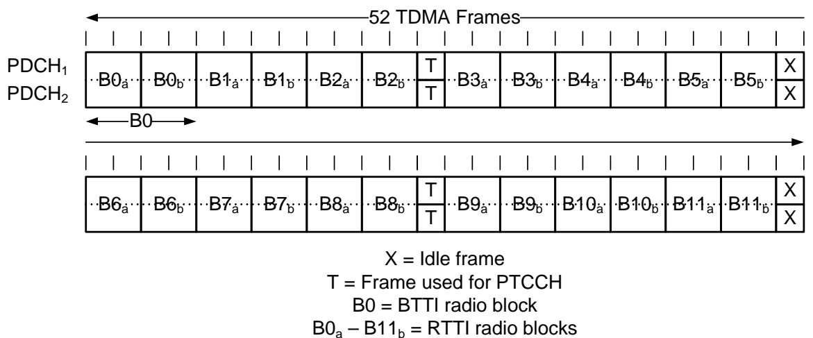
Figure 2a3: 52- multiframe for a PDCH-pair in RTTI configuration.
