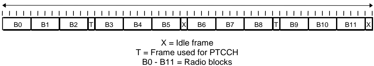
Figure 2a1: 52- multiframe for PDCH/Fs in BTTI configuration.
