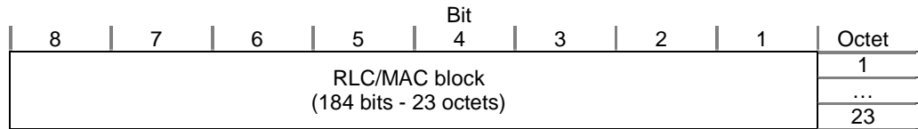
Figure 12.7.1.1: FACCH/SDCCH block
