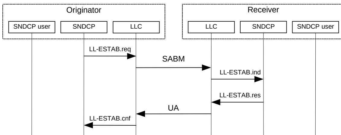
Figure 6: SNDSCP-initiated establishment / re-establishment
