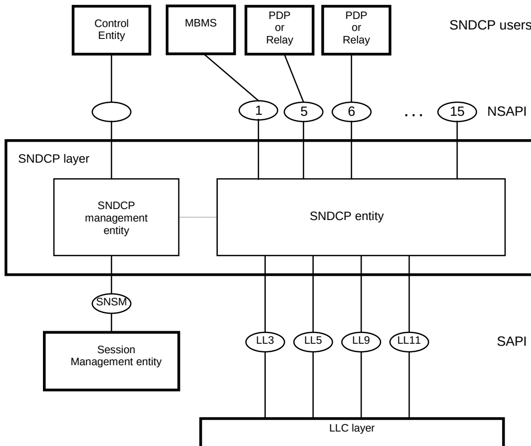
Figure 3: Service Access Points provided and used by SNDSCP
