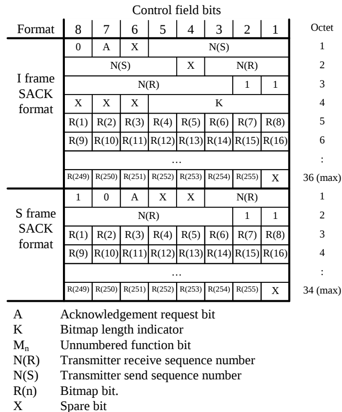
Figure 9: SACK I and S frame control field format
