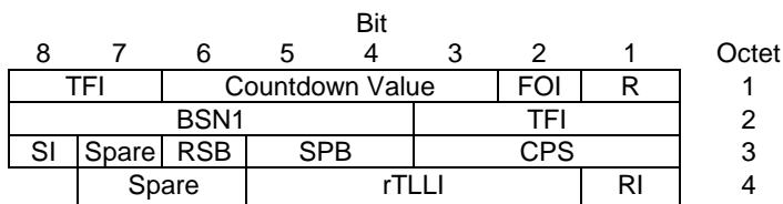
Figure 10.3a.4.3.3: EC-EGPRS uplink RLC data block header for MCS-1, MCS-2, MCS-3 and MCS-4
