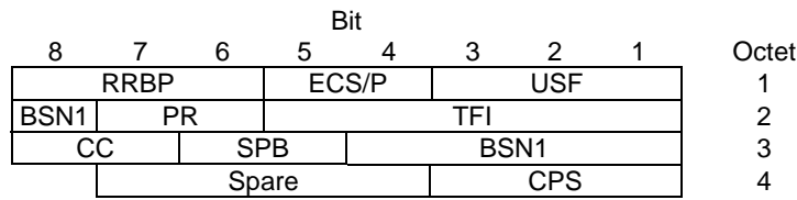
Figure 10.3a.3.3.6: EC-EGPRS downlink RLC data block header for MCS-1, MCS-2, MCS-3 and MCS-4
