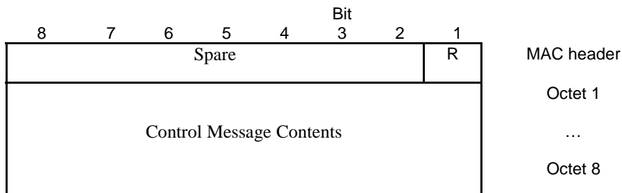
Figure 10.3.2.2: EC-EGPRS Uplink RLC/MAC control block together with its MAC header.
