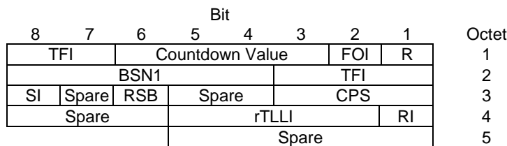
Figure 10.3a.4.2.3: EC-EGPRS uplink RLC data block header for MCS-5 and MCS-6
