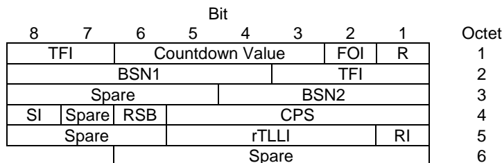
Figure 10.3a.4.1.3: EC-EGPRS uplink RLC data block header for MCS-7, MCS-8 and MCS-9.
