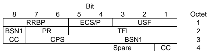
Figure 10.3a.3.2.5: EC-EGPRS downlink RLC data block header for MCS-5 and MCS-6
