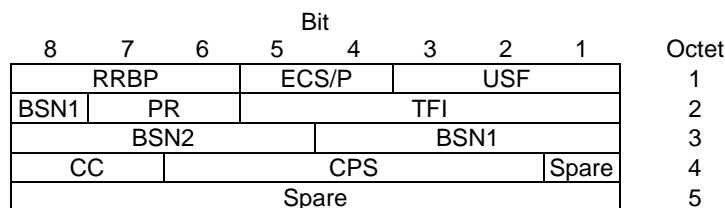
Figure 10.3a.3.1.5: EC-EGPRS downlink RLC data block header for MCS-7, MCS-8 and MCS-9
