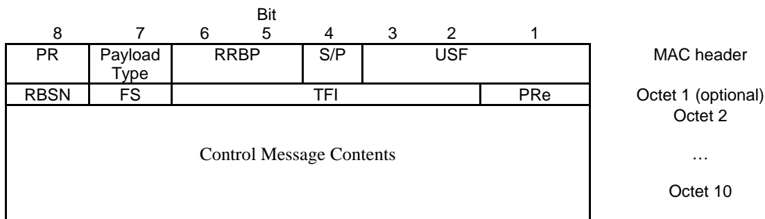
Figure 10.3.1.3.1: EC-EGPRS Downlink RLC/MAC control block together with its MAC header
