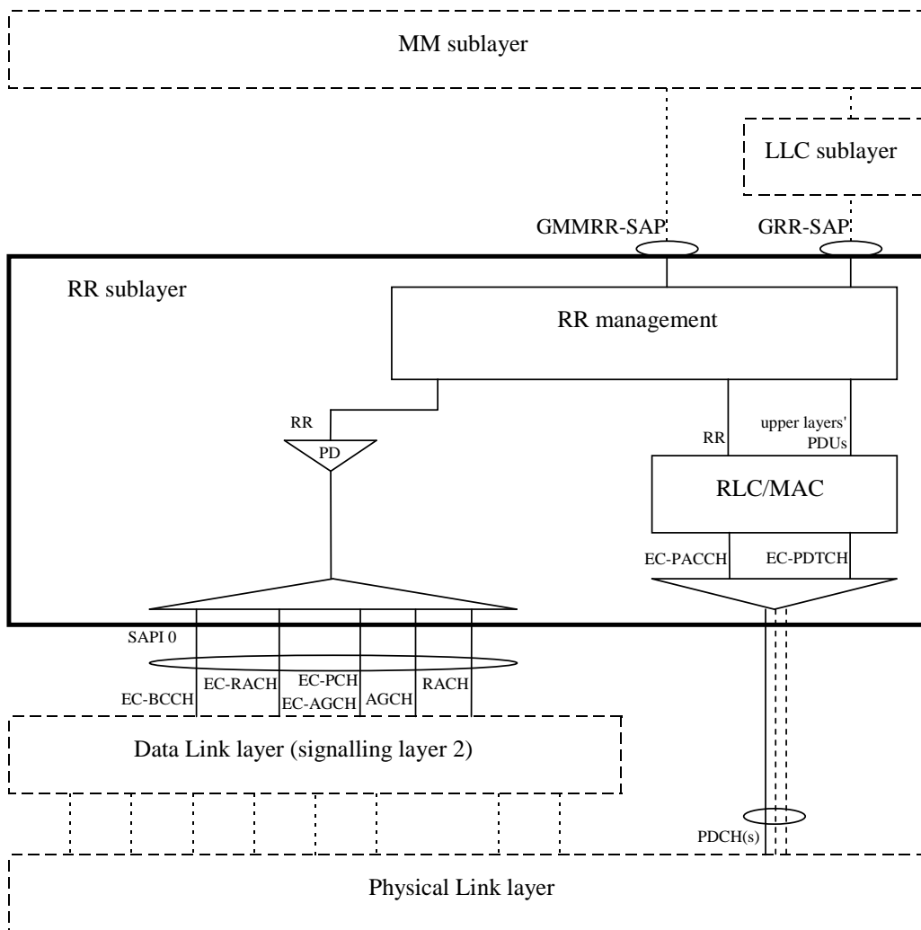
Figure 4.2: Protocol architecture of Radio Resource (RR) sublayer and RLC/MAC function in EC-EGPRS operation
