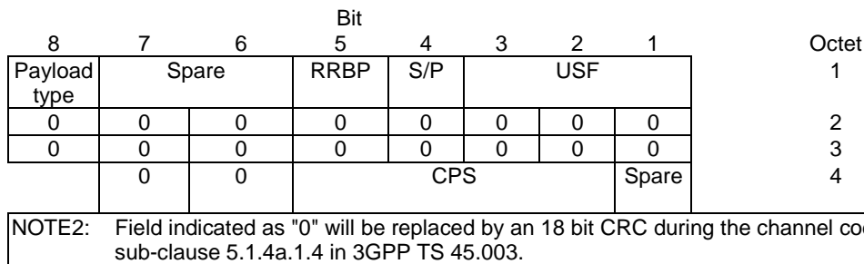
Figure 10.3a.3.3.3: Downlink RLC/MAC control block header for MCS-0.
