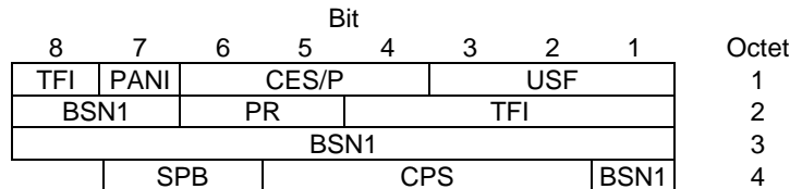
Figure 10.3a.3.3.2: EGPRS (FANR activated) / EGPRS2 downlink RLC data block header for MCS-1, MCS-2, MCS-3 and MCS-4
