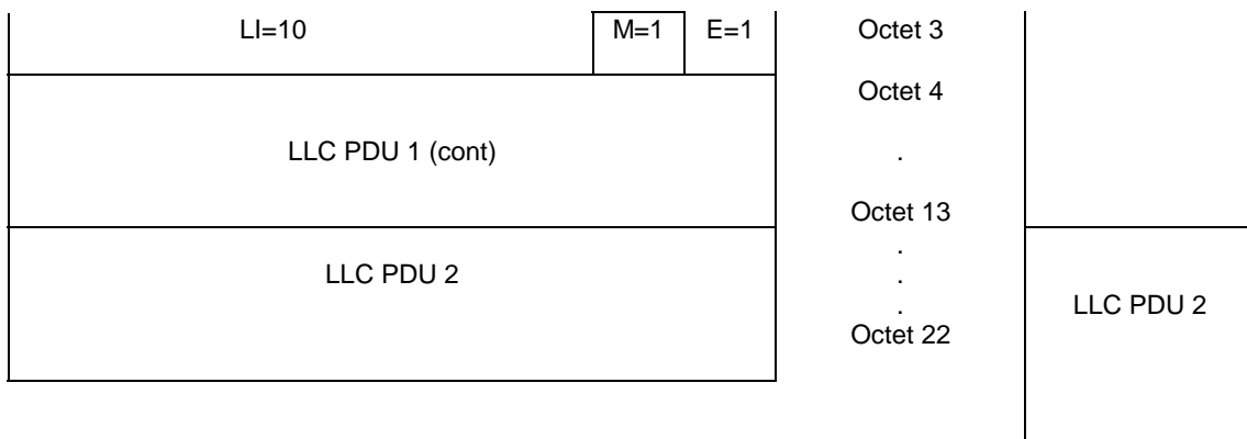
Figure B.7: Example when Length indicator (LI) can be omitted
