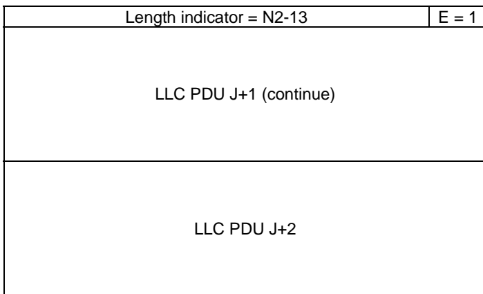
RLC Block with BSN=N-1 (mod SNS)
