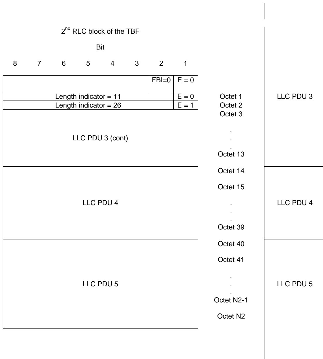
Figure B.8: Example for the case when a LLC PDU stretches over more than 2 consecutive in sequence RLC data blocks (LLC PDU 3 and LLC PDU 5).
