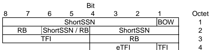
Figure 10.3a.5.2: Uplink Piggy-backed Ack/Nack field (SSN-based, eTFI assigned)
