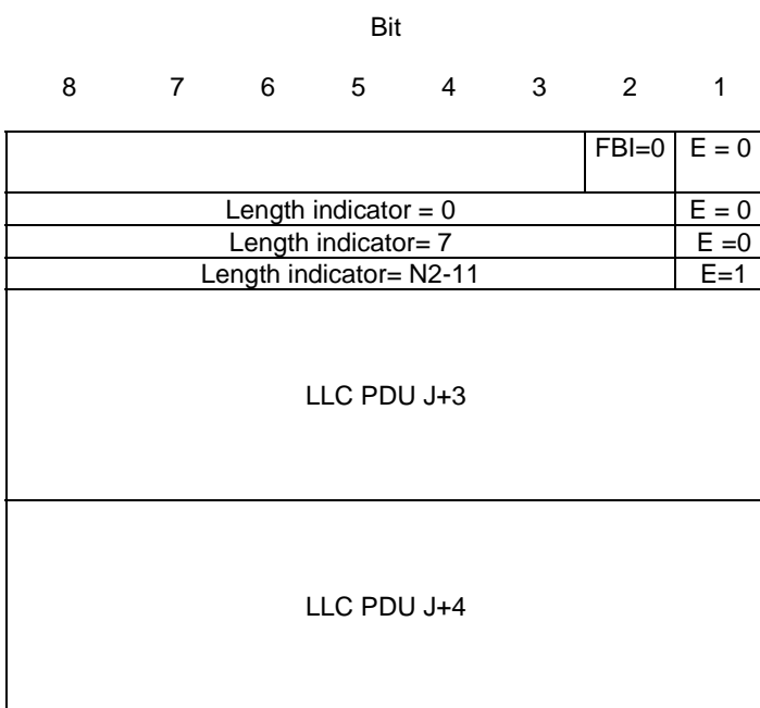
RLC Block with BSN=N-1 (mod SNS)
