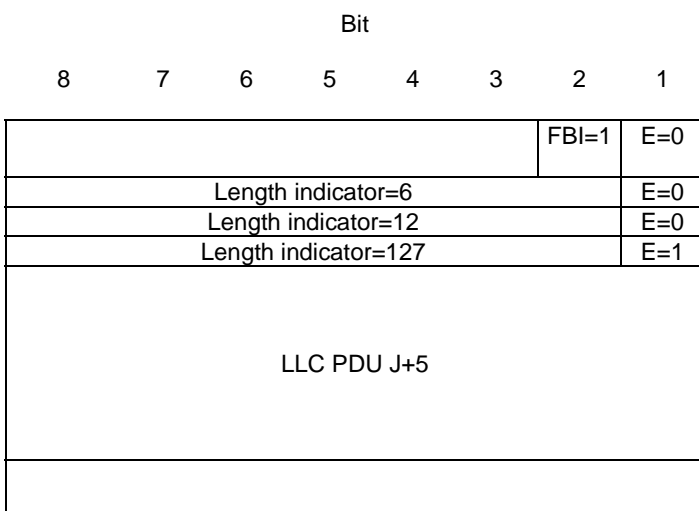
RLC Block with BSN=N (mod SNS)
