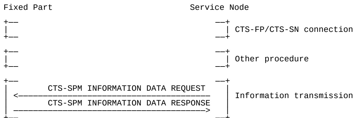
Figure 5.4/GSM 04.xx: Information request procedure
