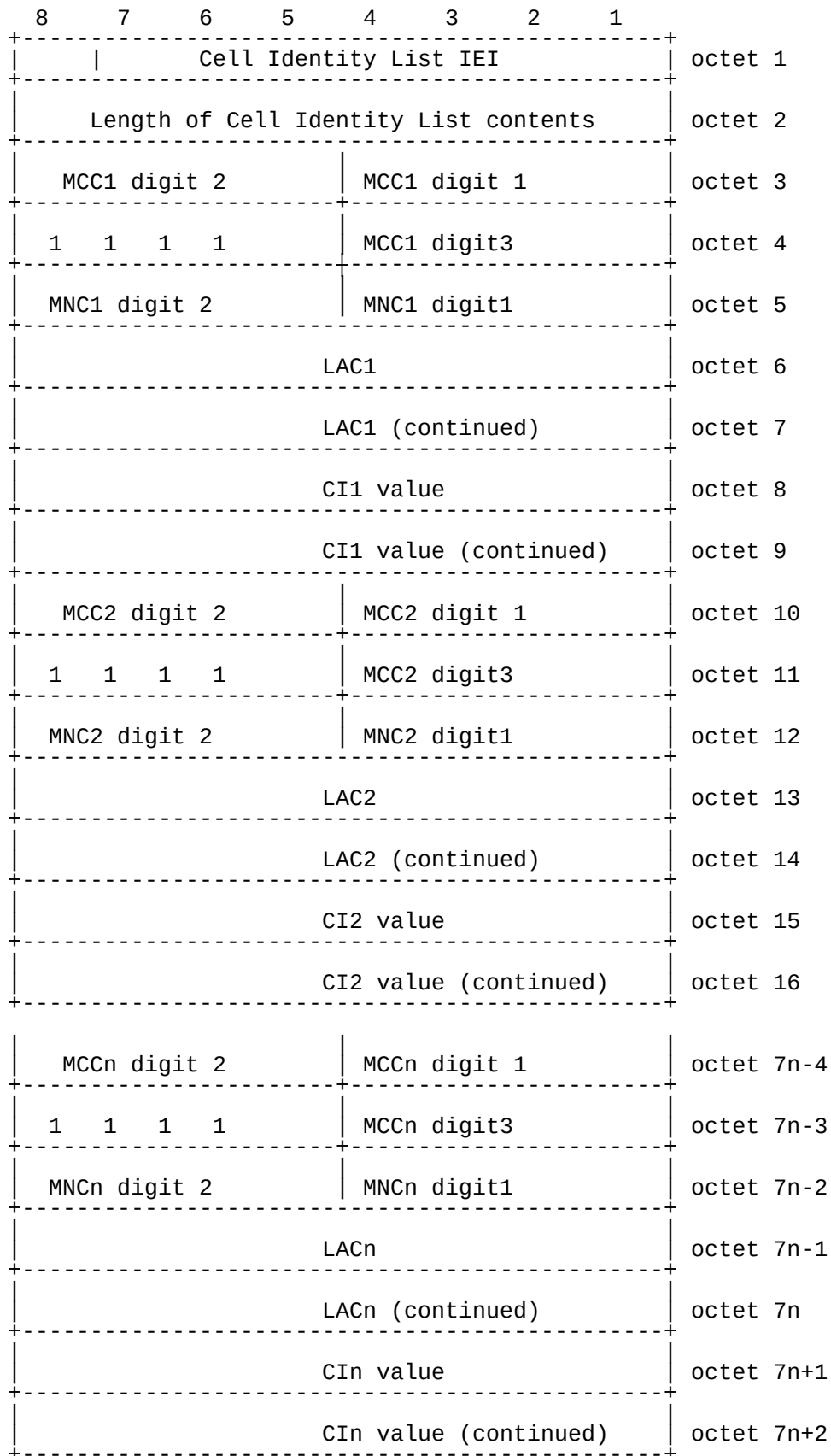
Figure 10.5/GSM 04.xx: Cell Identity List information element
