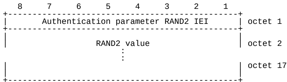
Figure 10.x/GSM 04.xx: Authentication Parameter RAND2 information element
