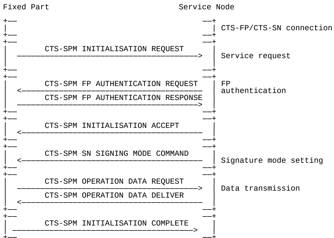
Figure 5.1/GSM 04.xx: CTS-FP initialisation
