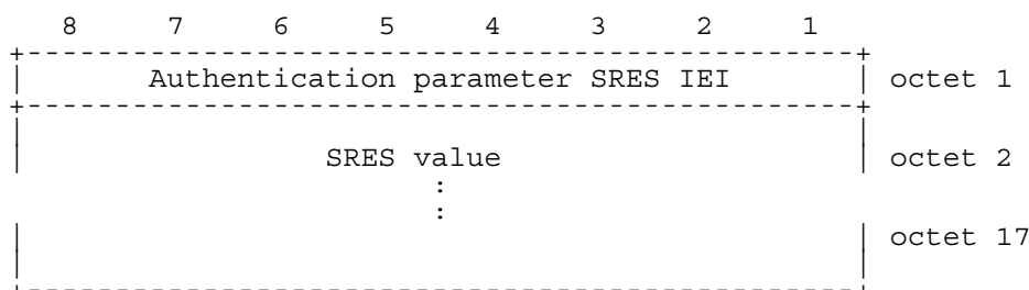
Figure 10.x/GSM 04.xx Authentication Parameter SRES information element
