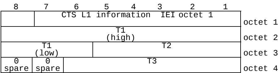
Figure 10.5/GSM 04.56: CTS L1 information information element
