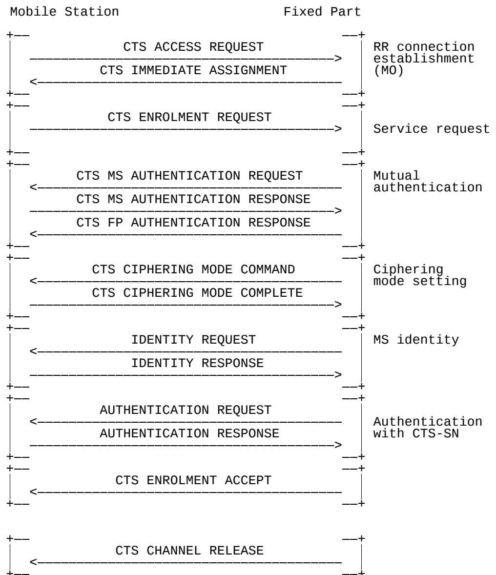
Figure 7.5/GSM 04.56: CTS enrolment
