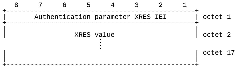
Figure 10.15/GSM 04.56: Authentication Parameter XRES information element
