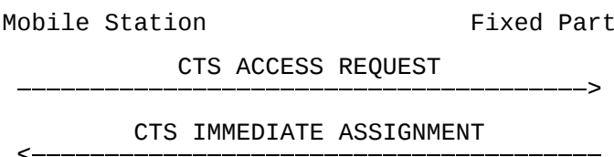
Figure 7.2/GSM 04.56: CTS immediate assignment
