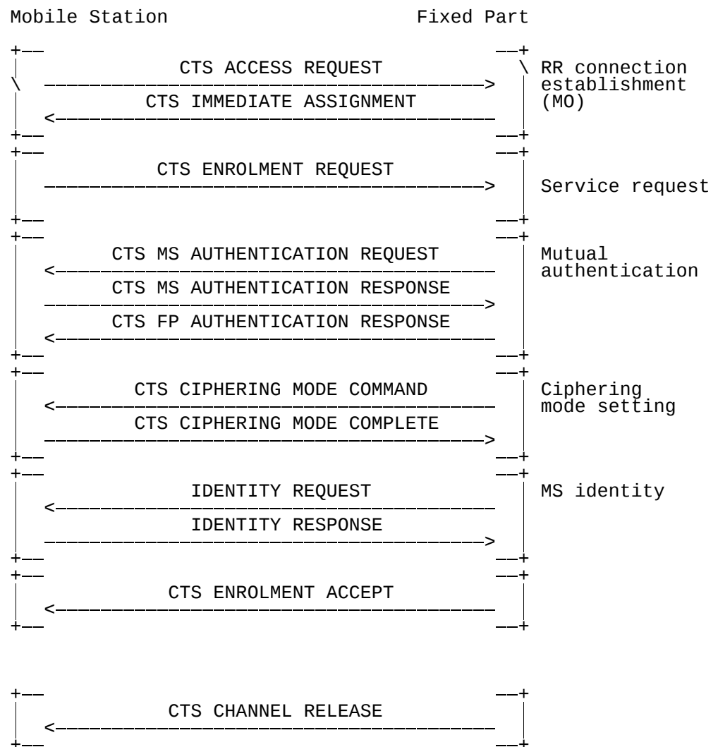
Figure 7.4/GSM 04.56: CTS enrolment
