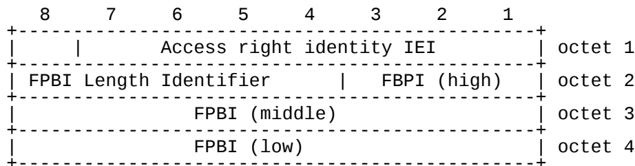
Figure 10.20/GSM 04.56: Access right identity information element
