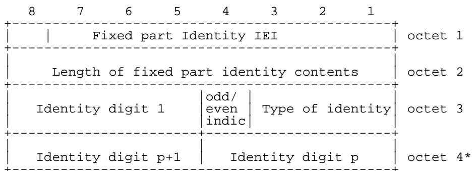
Figure 10.17/GSM 04.56: Fixed part Identity information element
