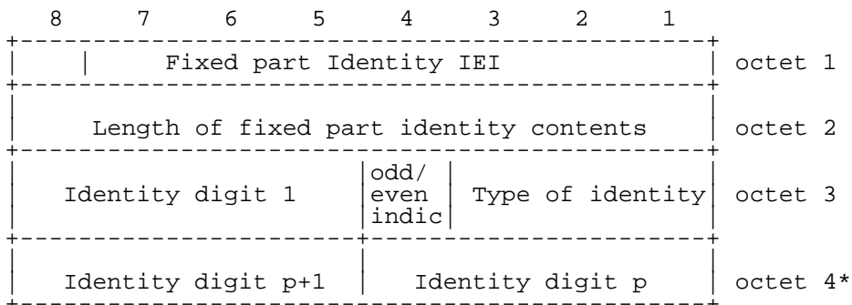
Figure 10.17/GSM 04.56: Fixed part Identity information element
