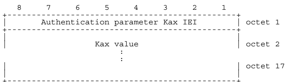
Figure 10.16/GSM 04.56: Authentication Parameter Kax information element
