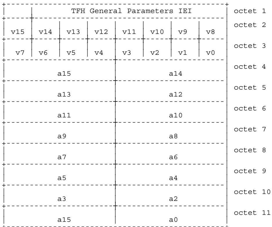
Figure 10.2/GSM 04.56: TFH General Parameters information element
