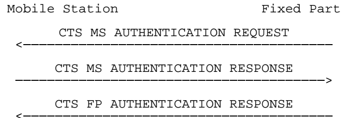
Figure 7.3/GSM 04.56: CTS mutual authentication
