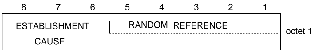
Figure 9.1.45.1: UPLINK ACCESS message content
