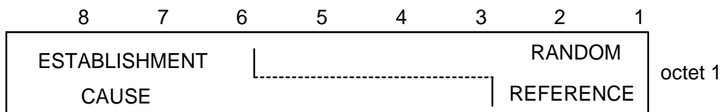
Figure 9.1.8.1: CHANNEL REQUEST message content
