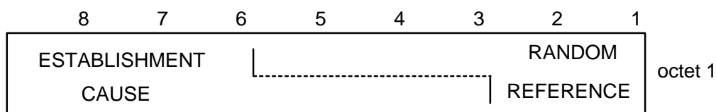
Figure 9.1.8.1: CHANNEL REQUEST message content
