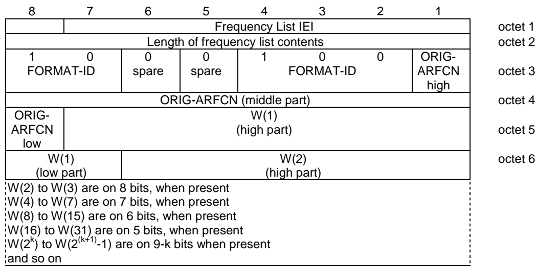
Figure 10.5.2.13.4.1: Frequency List information element (Range 512 format)
