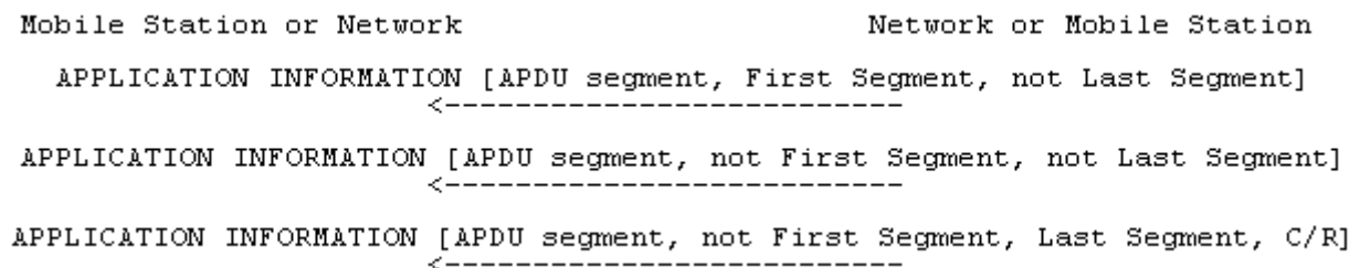
Figure 3.4.21.3.2.1: Application Information Transfer with segmentation
