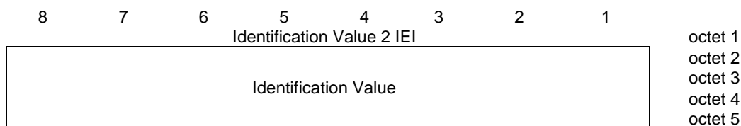
Figure 10.5.2.66.1: Token information element
