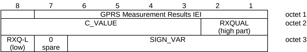
Figure 10.5.2.20a.1: GPRS Measurement Results information element
