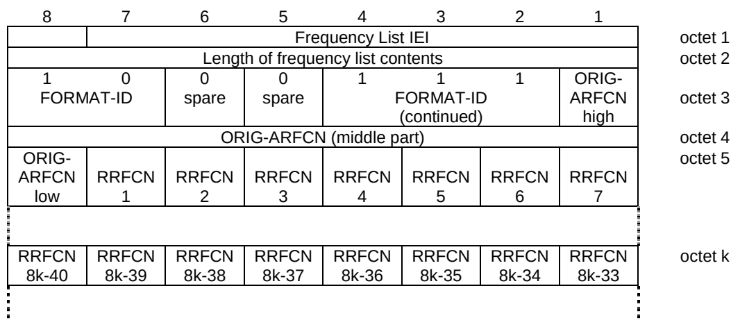
Figure 10.5.2.13.7.1: Frequency List information element, variable bit map format
