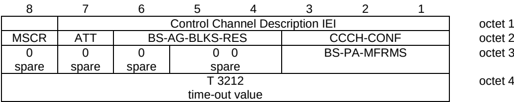
Figure 10.5.2.11.1: Control Channel Description information element
