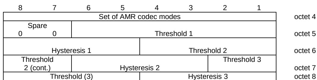
Figure 10.5.2.21aa.5: Parameters for multirate speech field for the MR version 1 when a set of four modes is chosen
