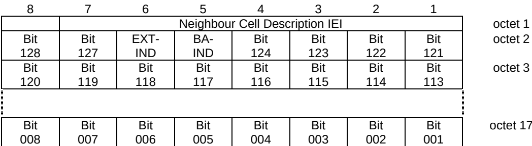
Figure 10.5.2.22.1: Neighbour Cell Description information element
