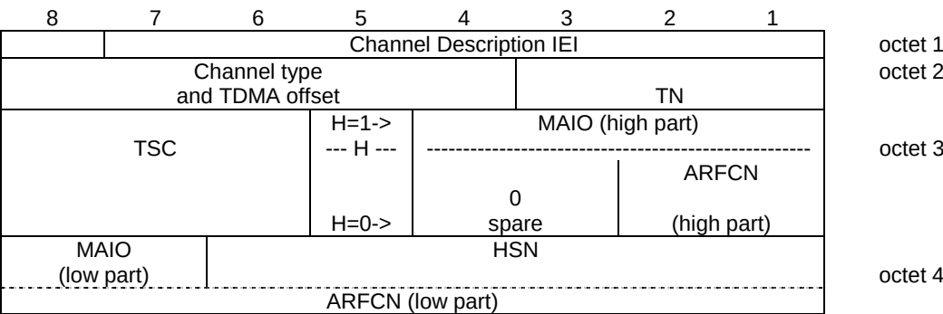
Figure 10.5.2.5.1: Channel Description information element
