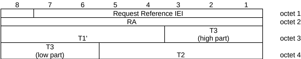
Figure 10.5.2.30.1: Request Reference information element
