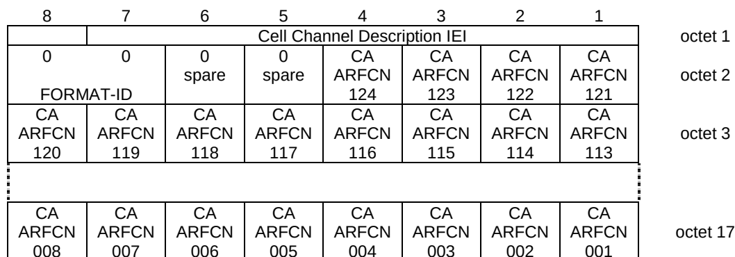
Figure 10.5.2.1b.2.1: Cell Channel Description information element, bit map 0 format
