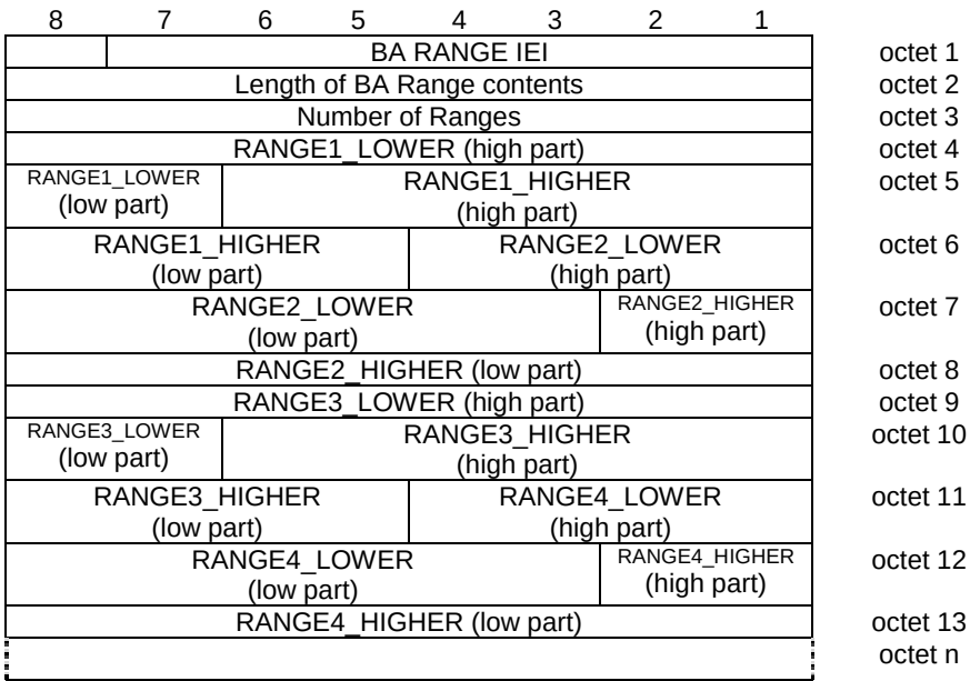
Figure 10.5.21a.1/3GPP TS 44.018: BA RANGE information element
