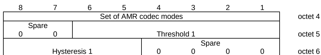
Figure 10.5.2.21aa.3/3GPP TS 04: Parameters for multirate speech field for the MR version 1 when a set with two codec modes is chosen
