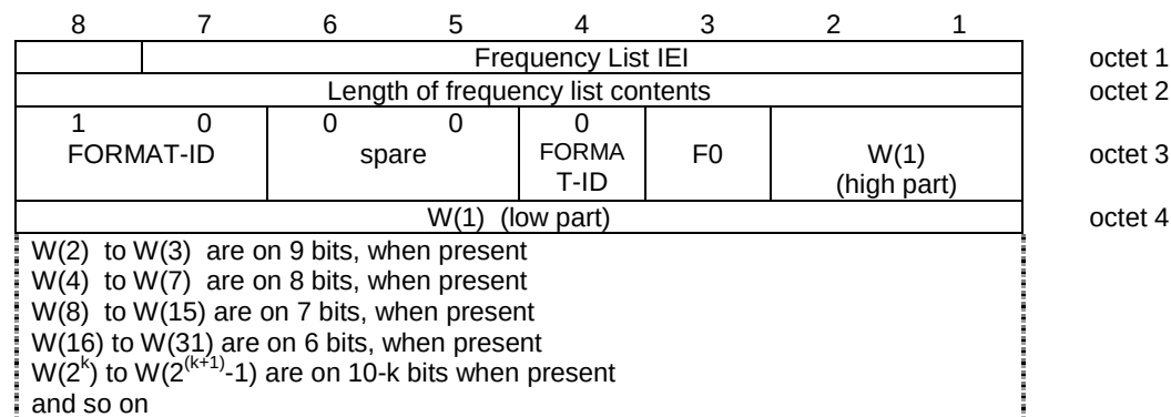
Figure 10.5.2.13.3.1/3GPP TS 44.018: Frequency List information element (Range 1024 format)
