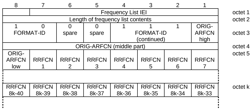
Figure 10.5.2.13.7.1/3GPP TS 44.018: Frequency List information element, variable bit map format
