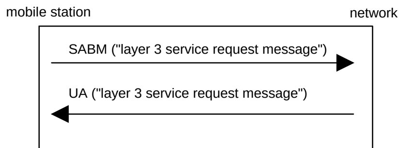
Figure 3.1.5.1/3GPP TS 44.018: Service request and contention resolution
