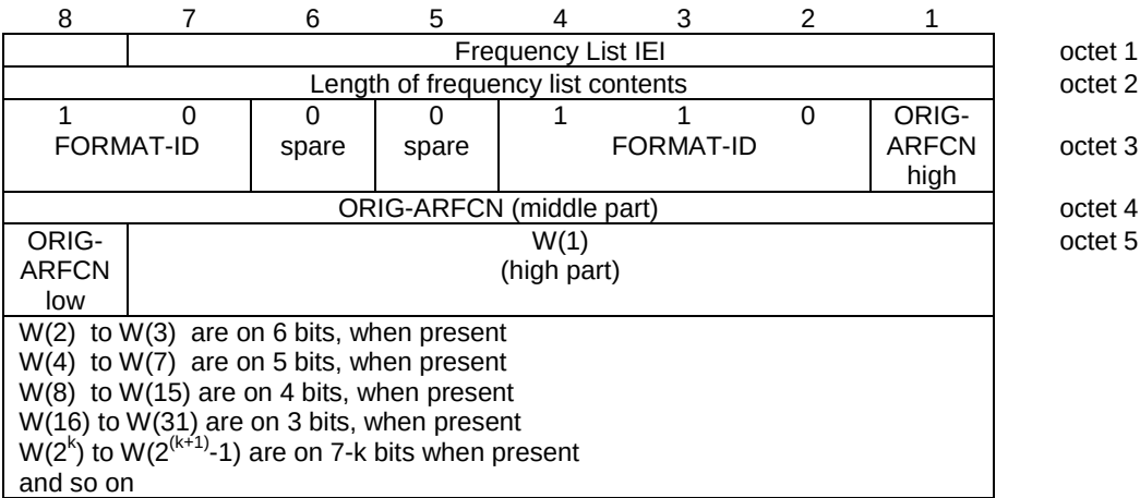
Figure 10.5.2.13.6.1/3GPP TS 44.018: Frequency List information element (Range 128 format)
