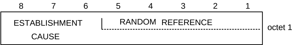
Figure 9.1.45.1/3GPP TS 44.018: UPLINK ACCESS message content
