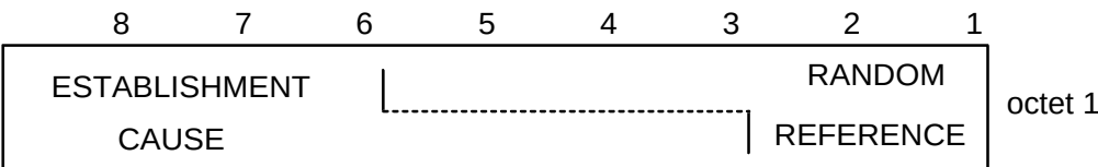
Figure 9.1.8.1/3GPP TS 44.018: CHANNEL REQUEST message content
