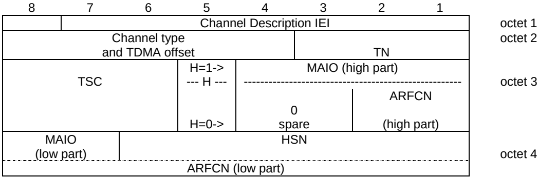
Figure 10.5.2.5a.1/3GPP TS 44.018: Channel Description 2 information element
