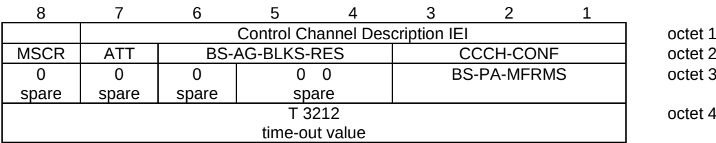
Figure 10.5.2.11.1/3GPP TS 44.018: Control Channel Description information element
