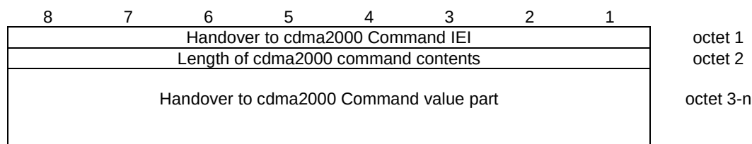
Figure 10.5.2.52.1/3GPP TS 44.018: Handover to cdma2000 Command information element
