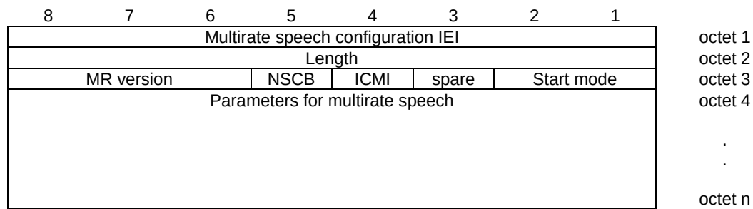
Figure 10.5.2.21aa.1/3GPP TS 44.018: MultiRate configuration information element
