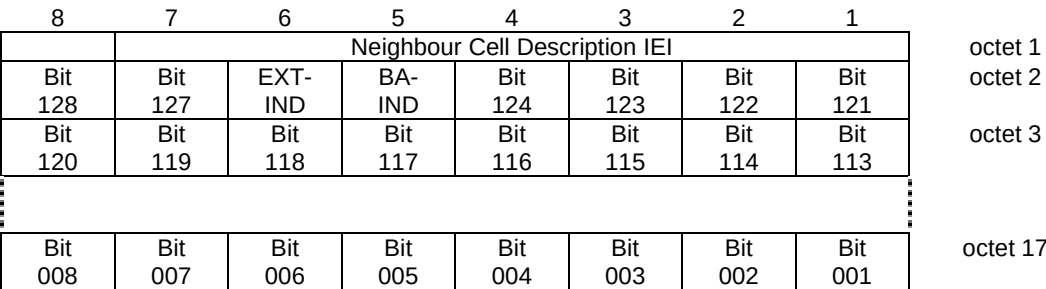
Figure 10.5.2.22.1/3GPP TS 44.018: Neighbour Cell Description information element
