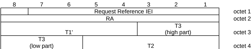
Figure 10.5.2.30.1/3GPP TS 44.018: Request Reference information element
