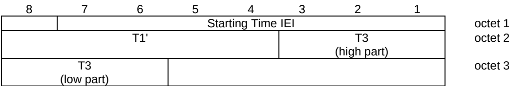
Figure 10.5.2.38.1/3GPP TS 44.018: Starting Time information element
