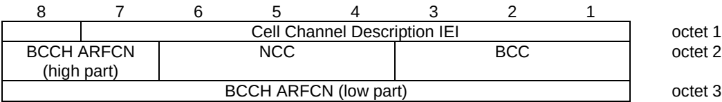
Figure 10.5.2.2.1/3GPP TS 44.018: Cell Description information element
