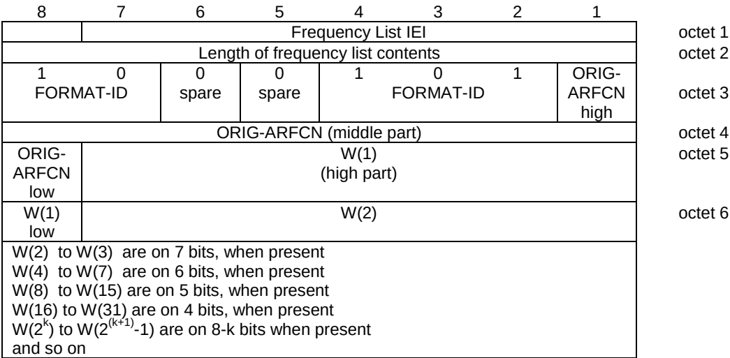
Figure 10.5.2.13.5.1/3GPP TS 44.018: Frequency List information element (Range 256 format)
