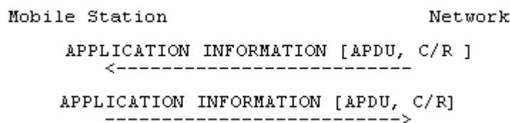
Figure 3.4.21.3.4.1/3GPP TS 44.018: Application Information Transfer without segmentation
