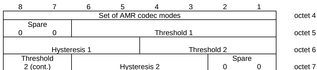
Figure 10.5.2.21aa.4/3GPP TS 44.018: Parameters for multirate speech field for the MR version 1 when a set of three codec modes is chosen
