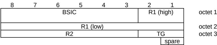
Figure 9.1.30b.1/3GPP TS 44.018: COMPACT Frame synchronization information element
