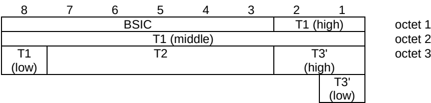
Figure 9.1.30a.1/3GPP TS 44.018: Frame synchronization information element
