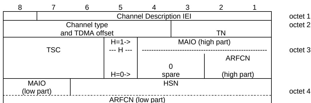
Figure 10.5.2.5.1/3GPP TS 44.018: Channel Description information element
