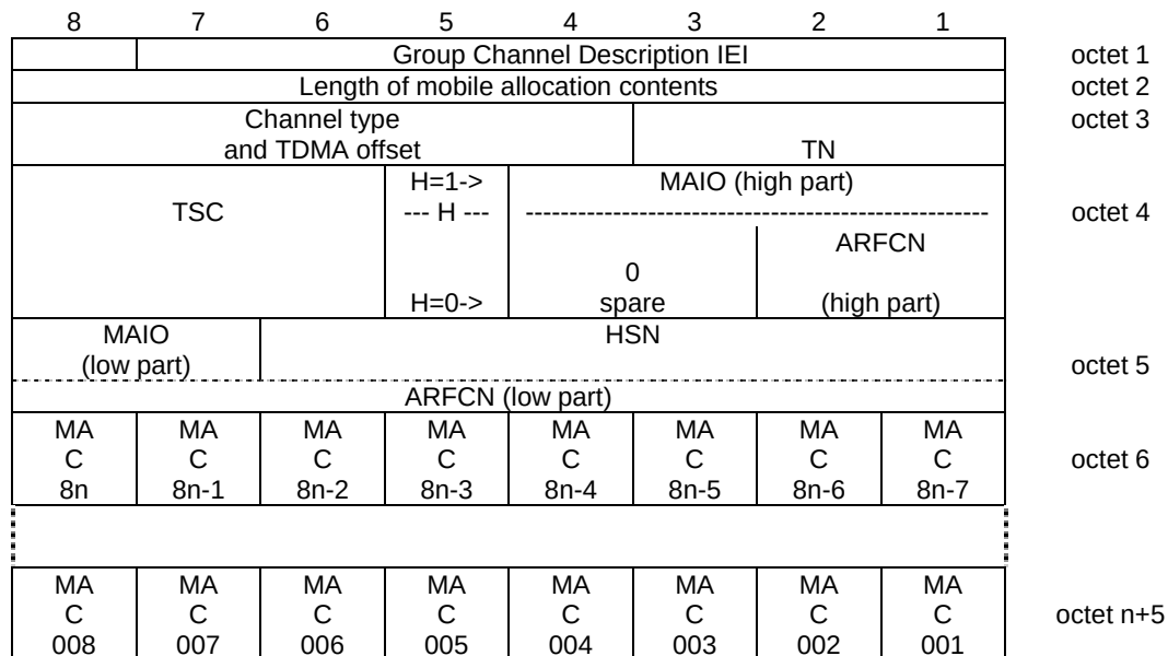
Figure 10.5.2.14b.1/3GPP TS 44.018: Group Channel Description information element
