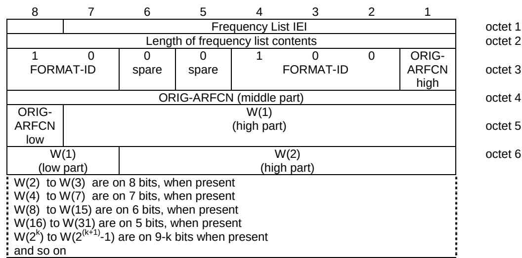
Figure 10.5.2.13.4.1/3GPP TS 44.018: Frequency List information element (Range 512 format)
