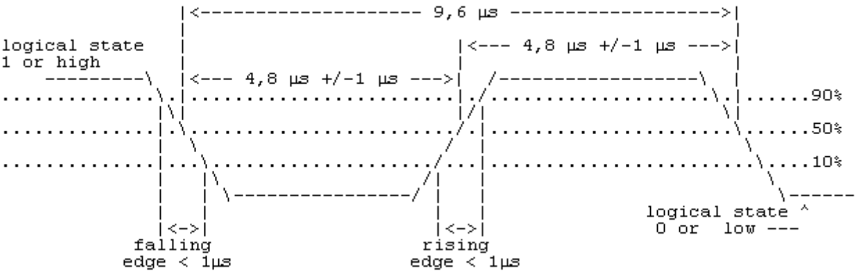
Figure 10.3.3: Timing characteristics
