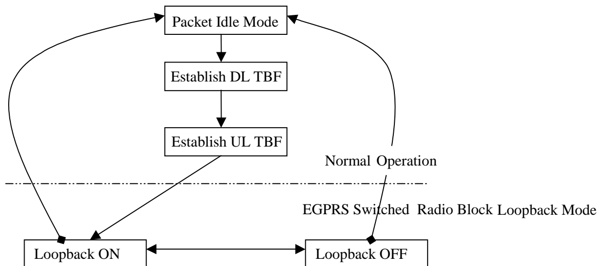
Figure 5.5.2: Loopback Sub-modes
