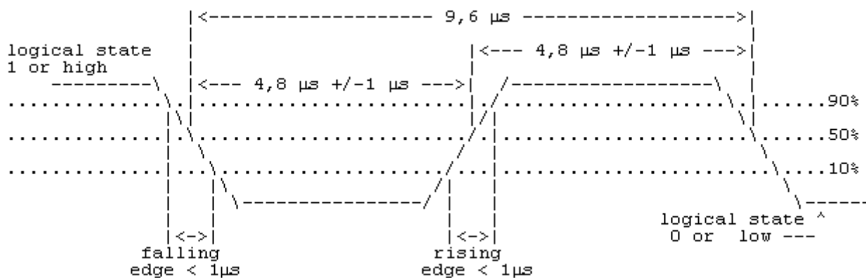
Figure 10.3.3: Timing characteristics
