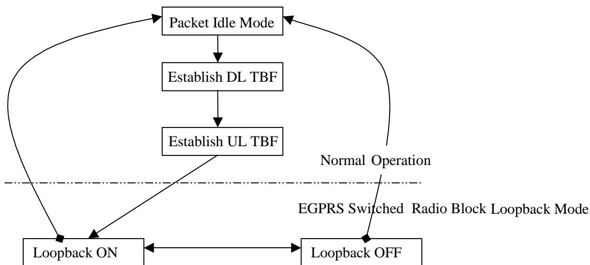
Figure 5.5.2: Loopback Sub-modes
