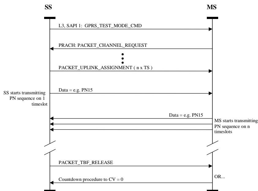
Figure 5.4.3: PN Sequence Definition
