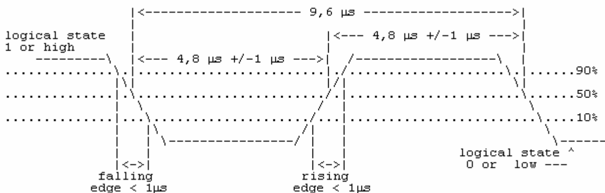
Figure 10.3.3: Timing characteristics
