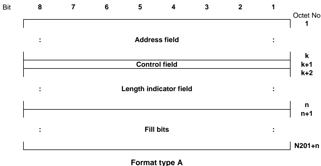
Figure 1/3GPP TS 04.06 (sheet 1 of 3): General frame formats
