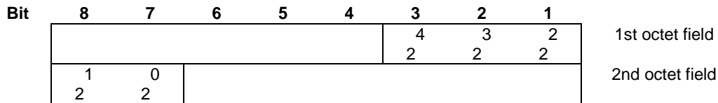
Figure 3/3GPP TS 04.06: Field mapping convention
