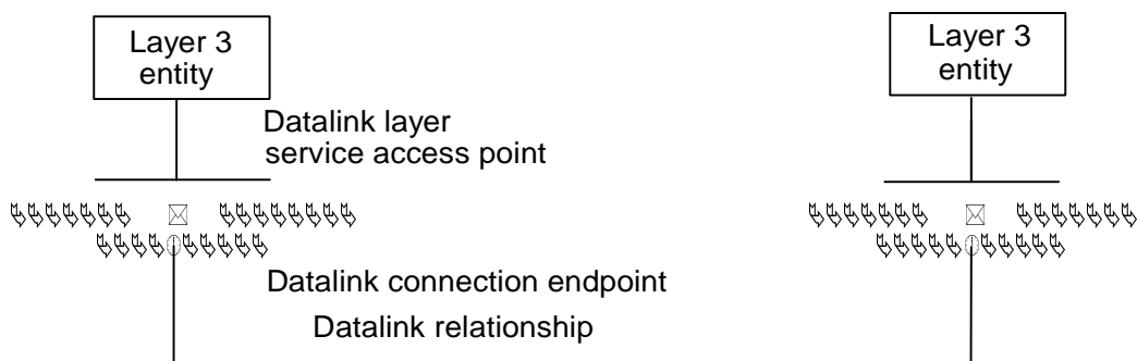
Figure 2: Peer-to-peer relationship
