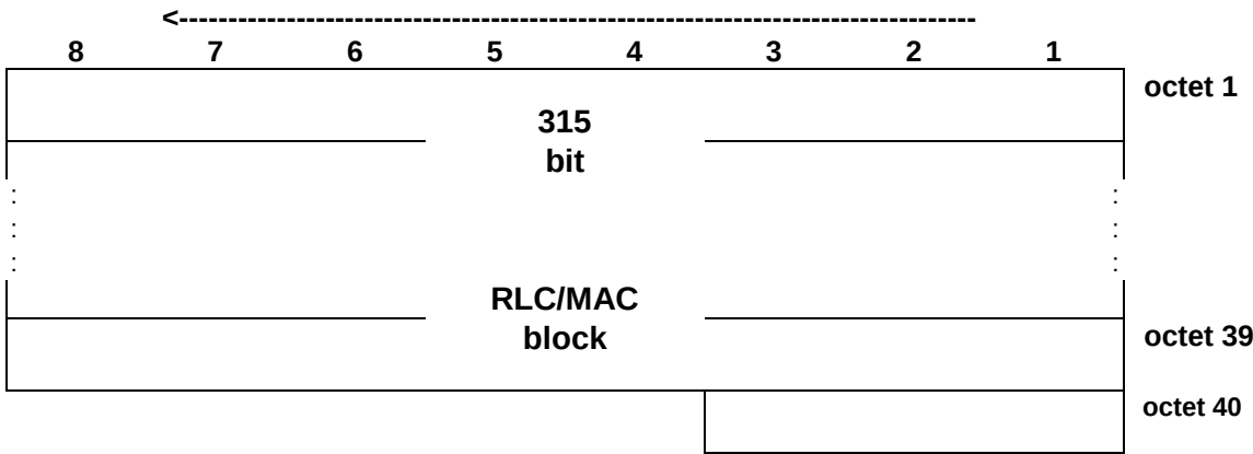
Figure 7.6.3: PDTCH block type 3 (CS-3) format
