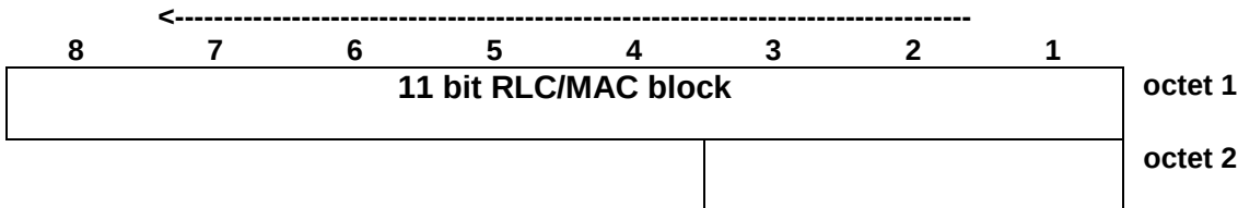
Figure 7.7.b: PRACH uplink/PACCH uplink short acknowledgement block format
