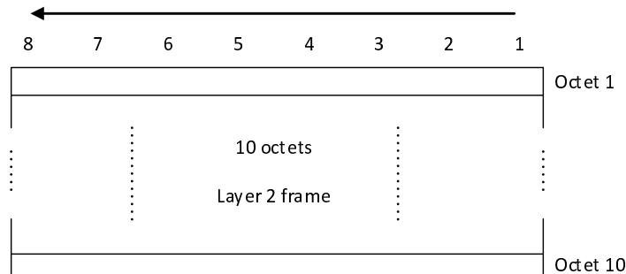
Figure 7.9b.2: EC-PACCH downlink block format
