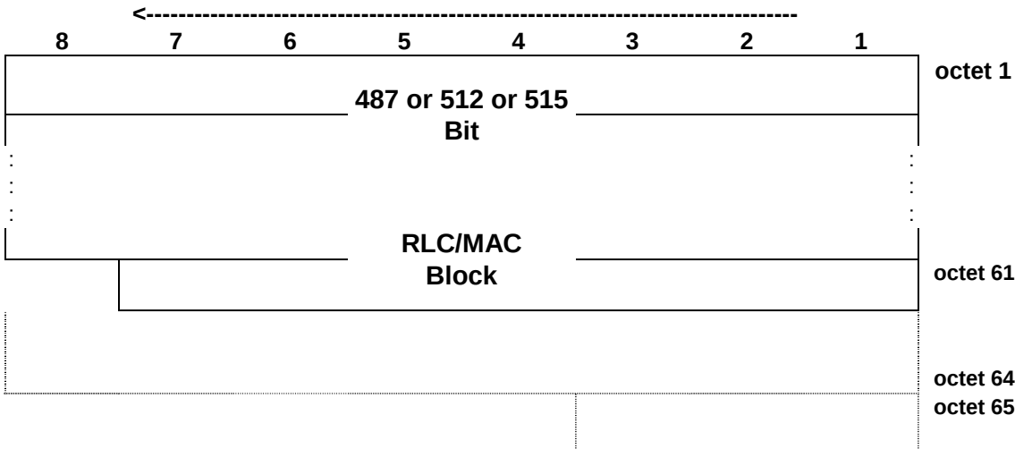
Figure 7.6.9.1: PDTCH block type 9 (MCS-5) uplink format
