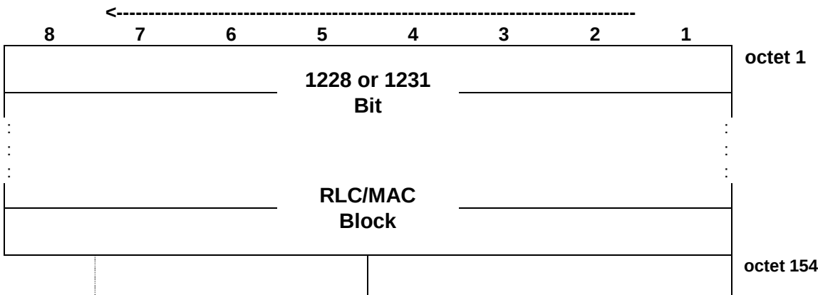
Figure 7.6.13.2: PDSCH block type 13 (MCS-9) downlink format
