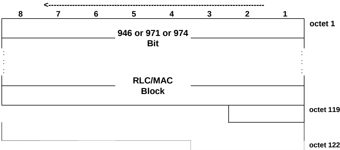
Figure 7.6.11.1: PDTCH block type 11(MCS-7) uplink format
