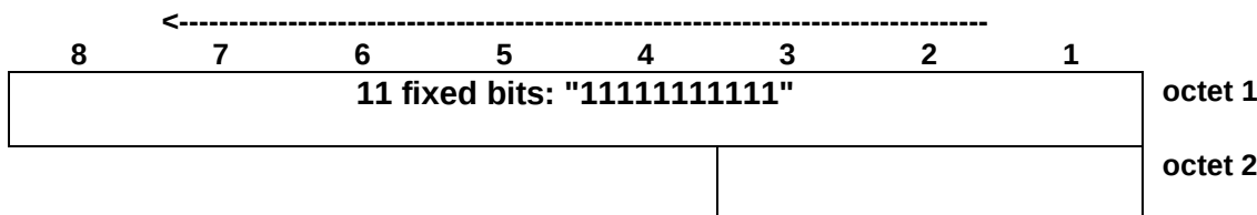
Figure 7.9.b: PTCCH uplink block format
