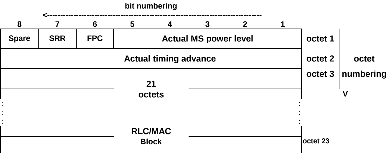
Figure 7.2.2: SACCH uplink block format for MS operating in Iu mode
