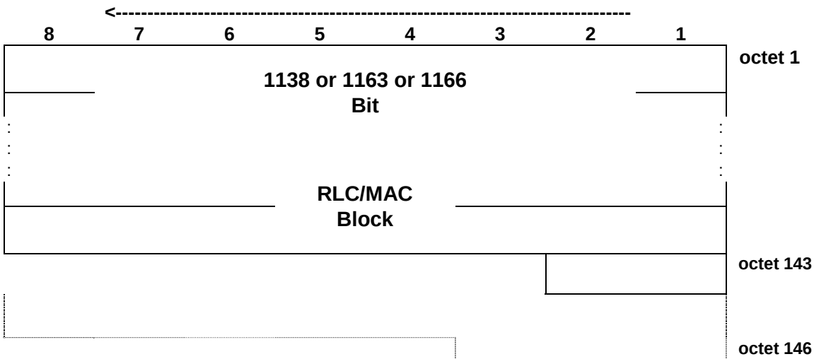
Figure 7.6.12.1: PDTCH block type 12 (MCS-8) uplink format
