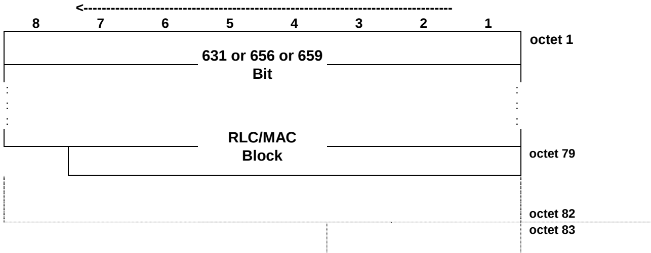
Figure 7.6.10.1: PDTCH block type 10 (MCS-6) uplink format
