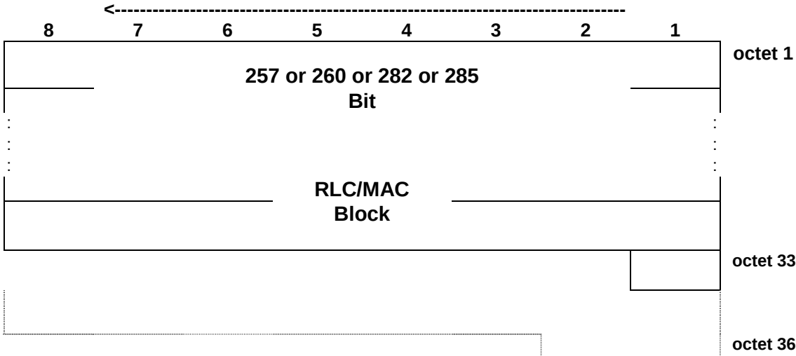
Figure 7.6.6: PTDCH block type 6 (MCS-2) format
