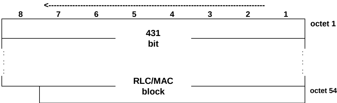
Figure 7.6.4: PDTCH block type 4 (CS-4) format
