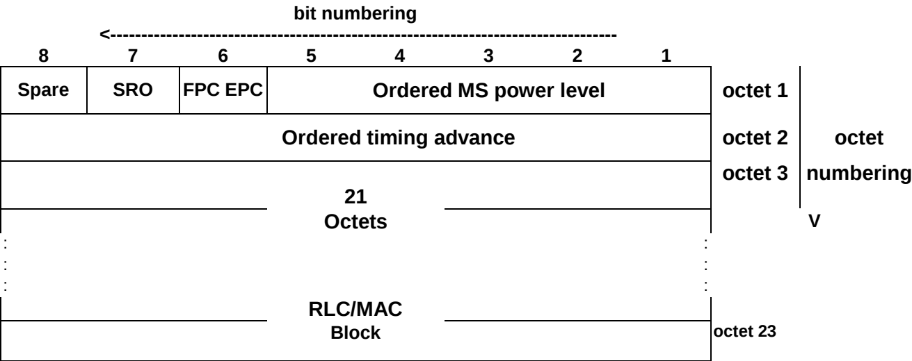
Figure 7.1.2: SACCH downlink block format for MS operating in Iu mode
