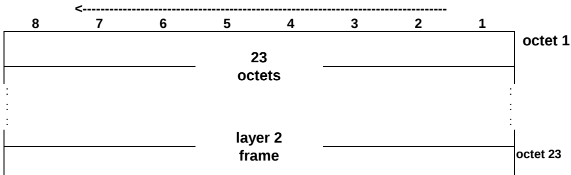
Figure 7.3.1: BCCH/CCCH/CBCH downlink block format
