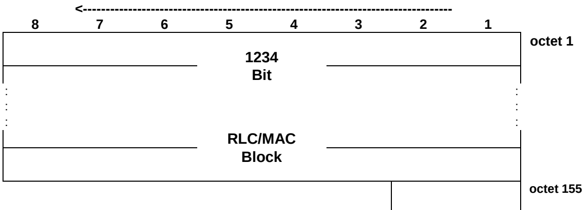
Figure 7.6.13.1: PDSCH block type 13 (MCS-9) uplink format
