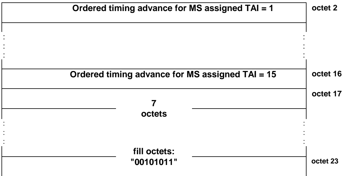
Figure 7.8: PTCCH downlink block format
