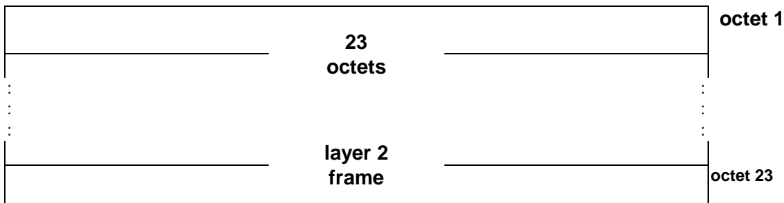
Figure 7.3.1: BCCH/CCCH/CBCH downlink block format
